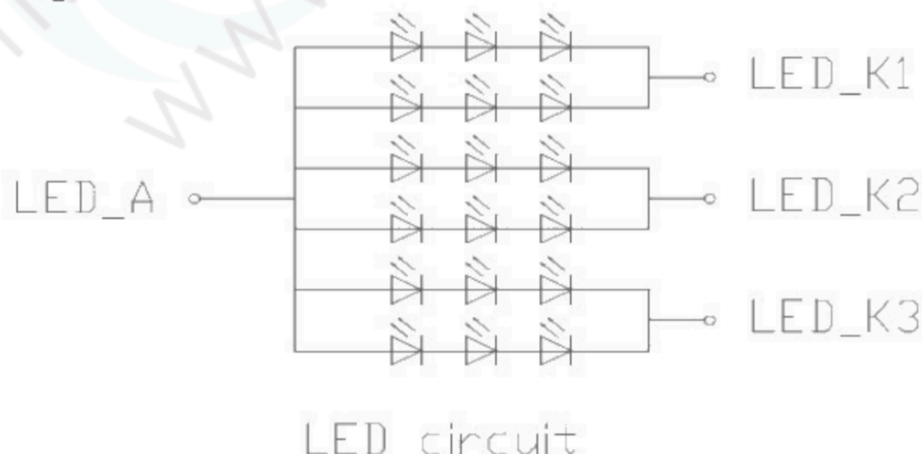
Figure 4.2 LED connection of backlight
