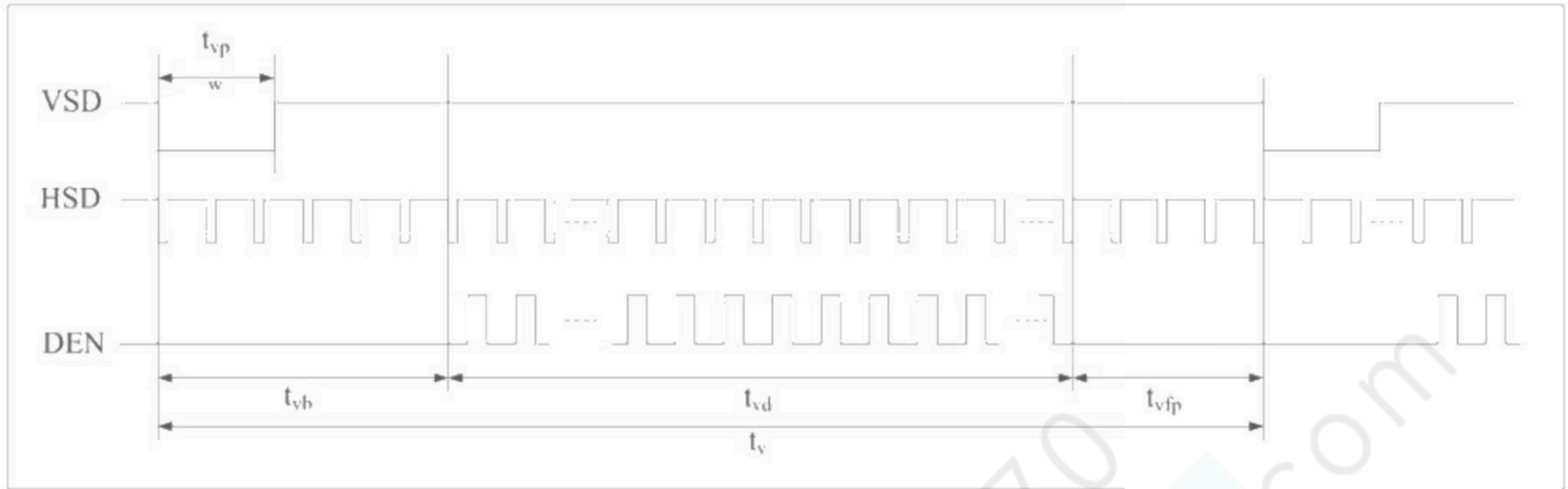
Figure 5.2.3 Vertical Input Timing Diagram
