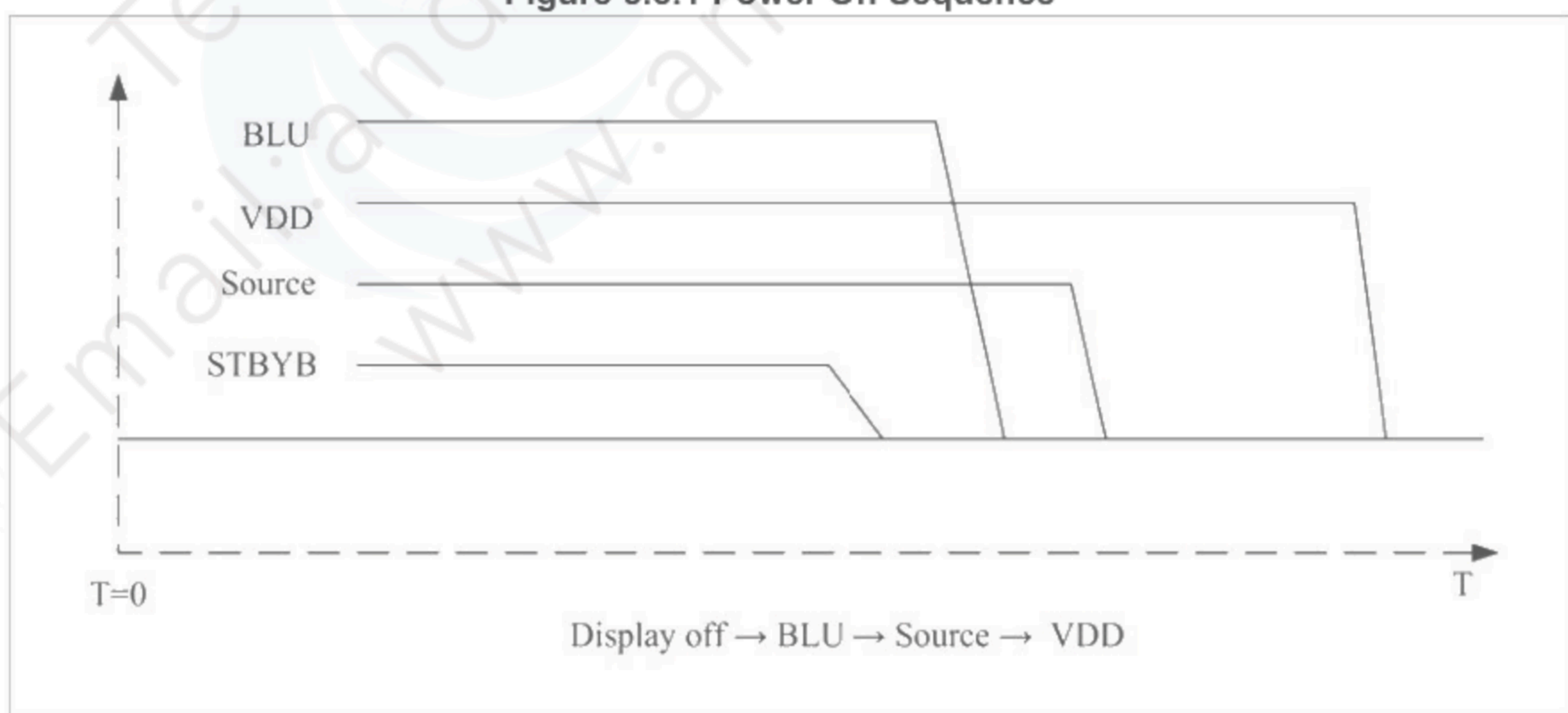
Figure 5.3.2 Power Off Sequence
