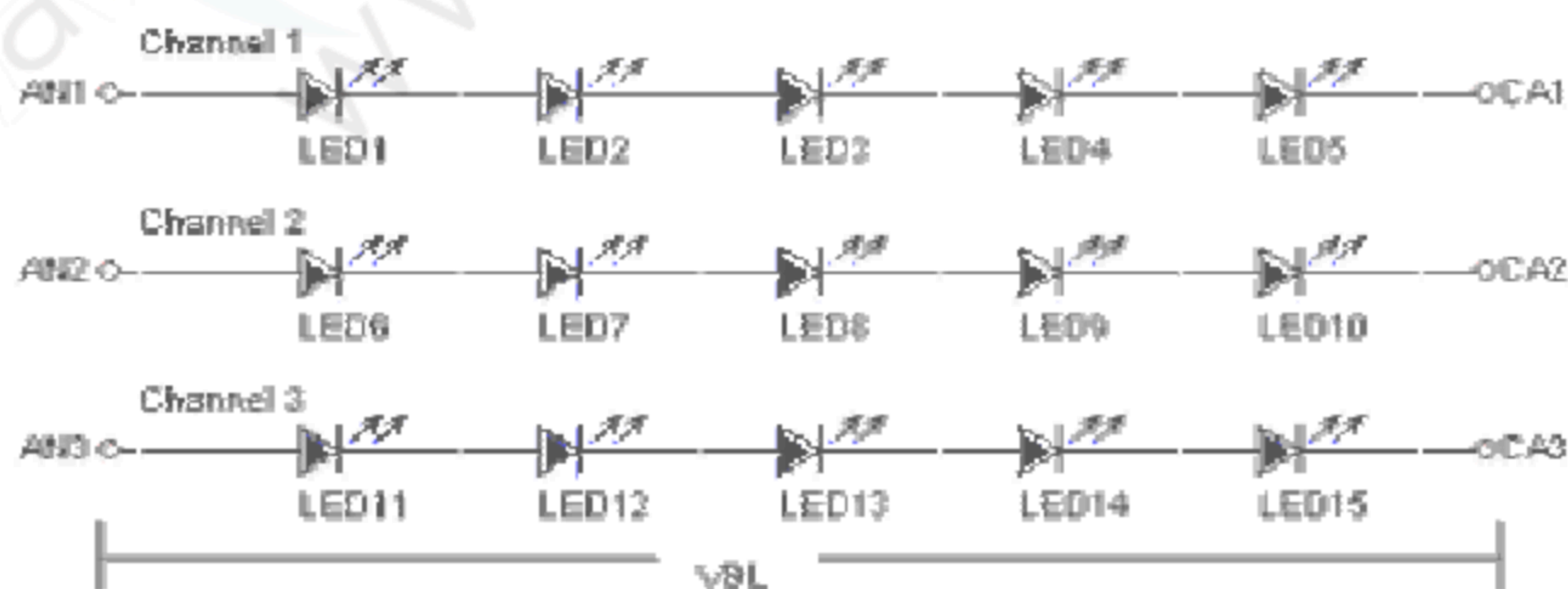
Figure 4.2 LED connection of backlight
