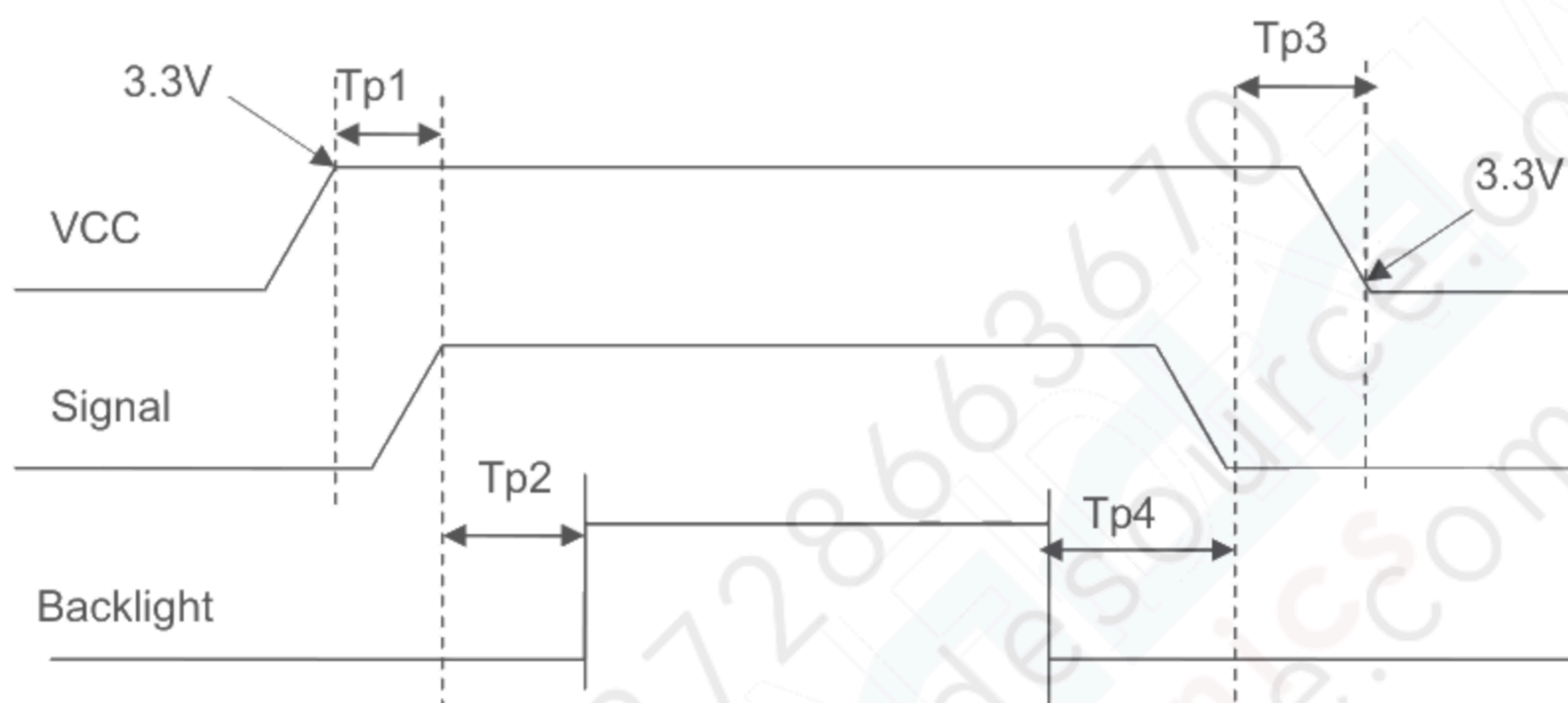
Figure 5.5 Power on/off sequence
