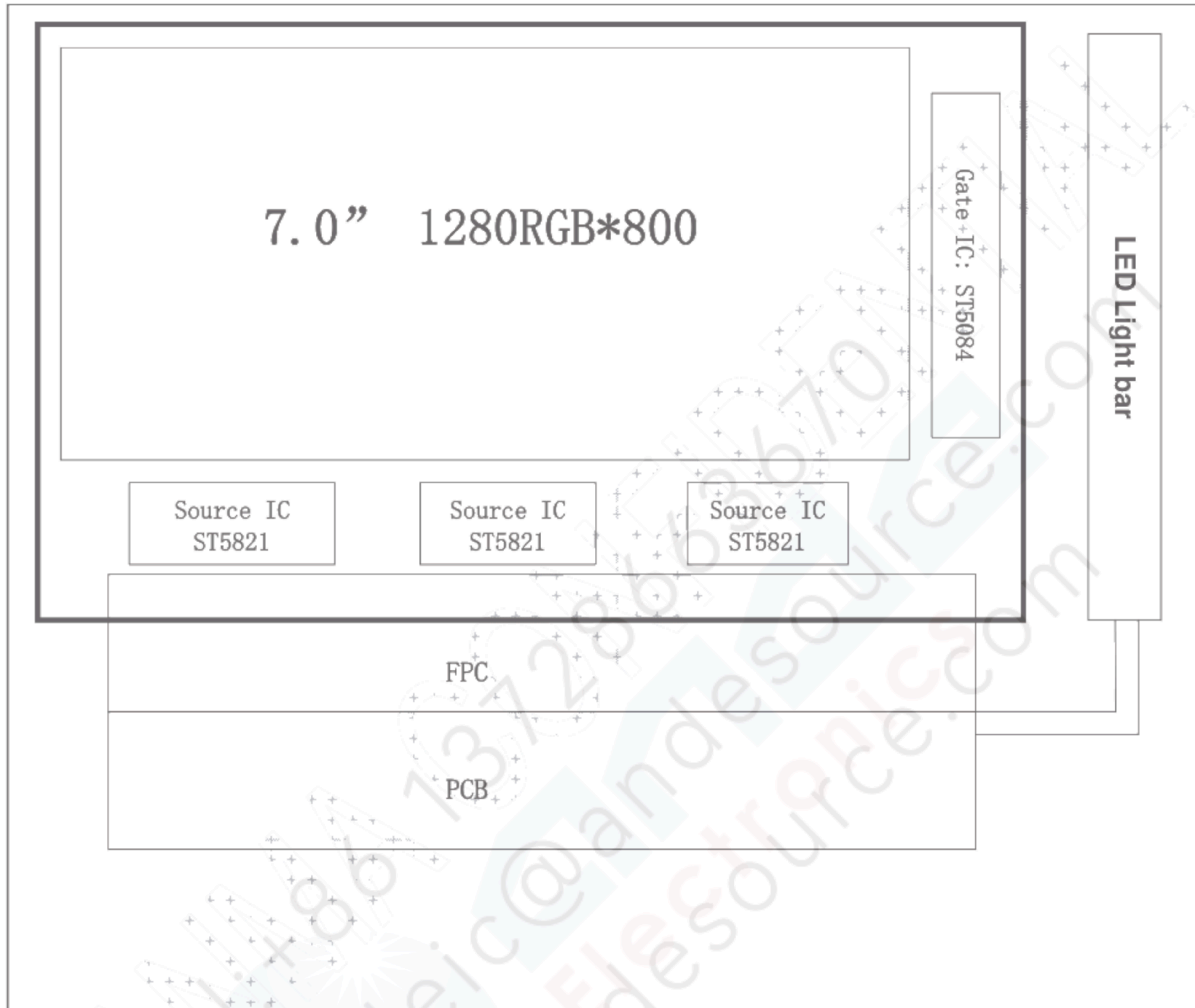
Figure 4.3 TFT Block Diagram
