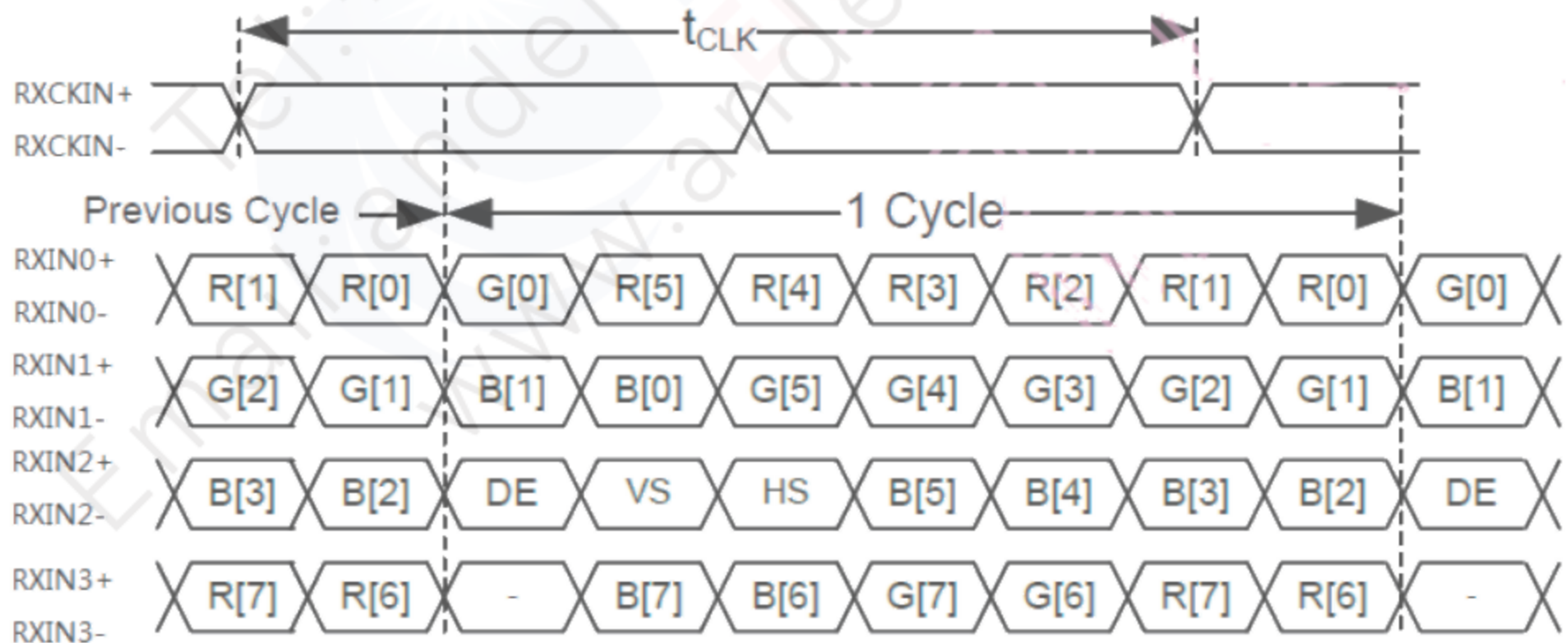
Figure 5.1 LVDS Input signal data timing
