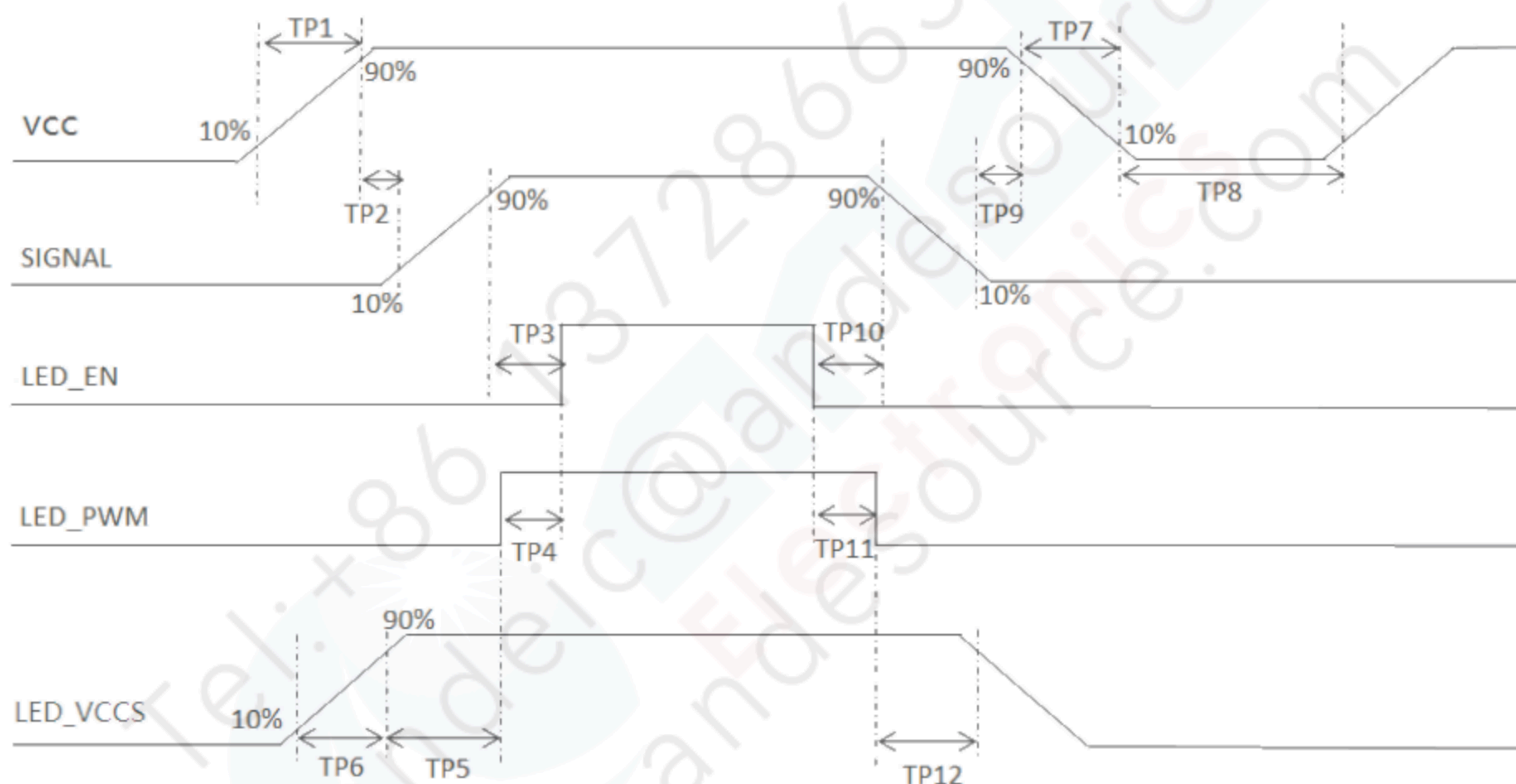
Figure 5.3 Power ON/OFF Sequence
