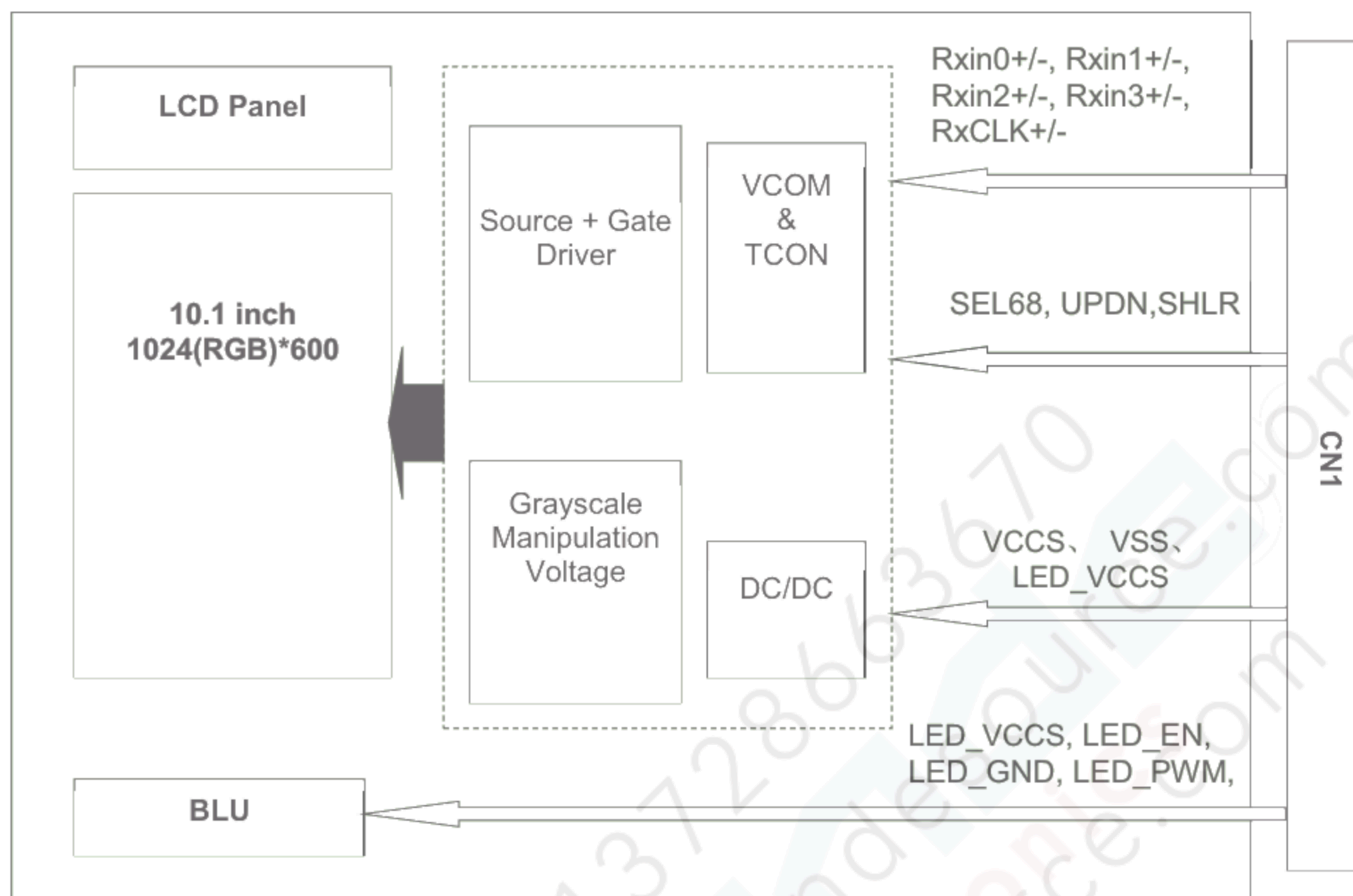
Figure 5.4 LCD Module Block Diagram
