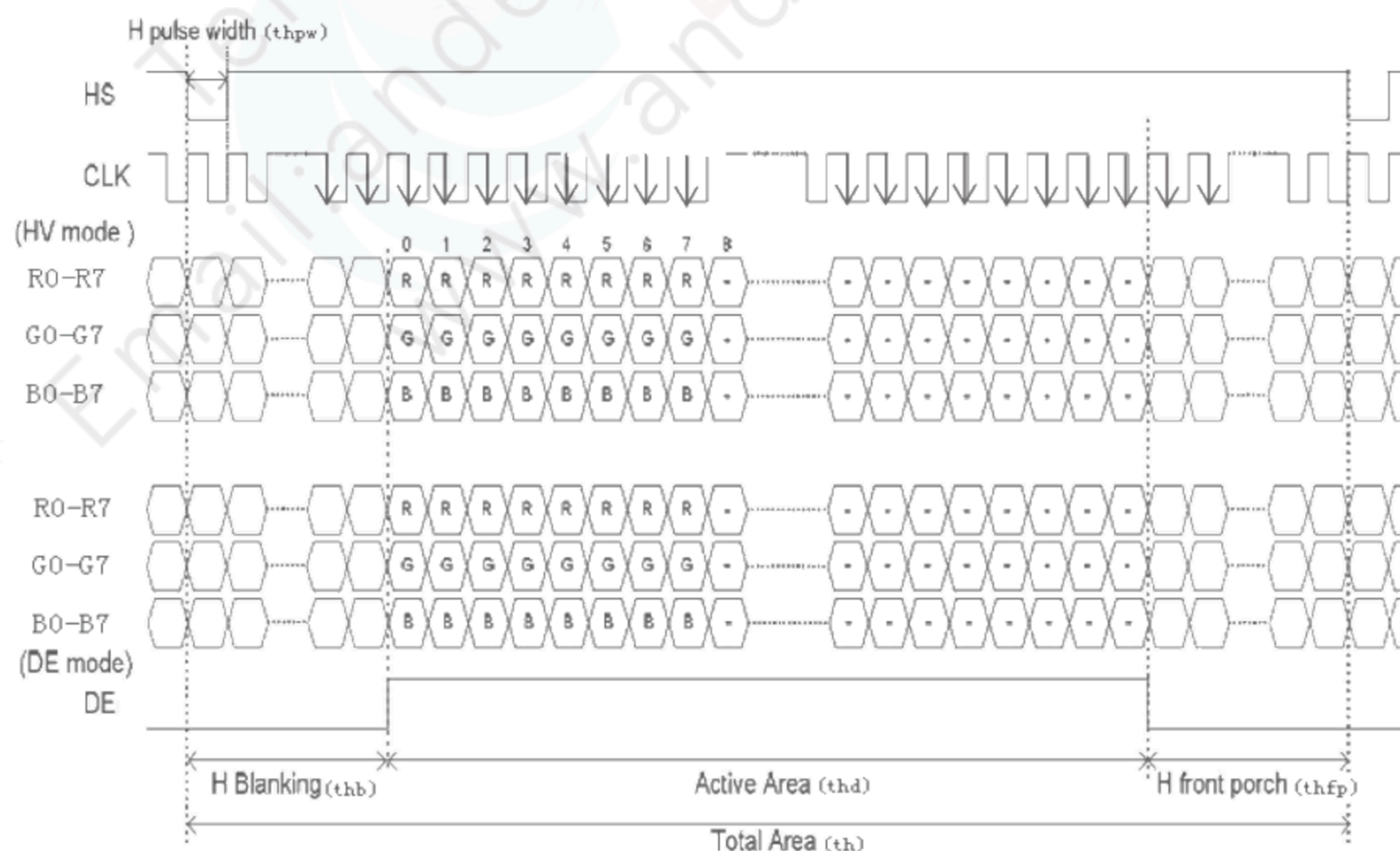
Figure 6.2.2 Vertical Input Timing Diagram
