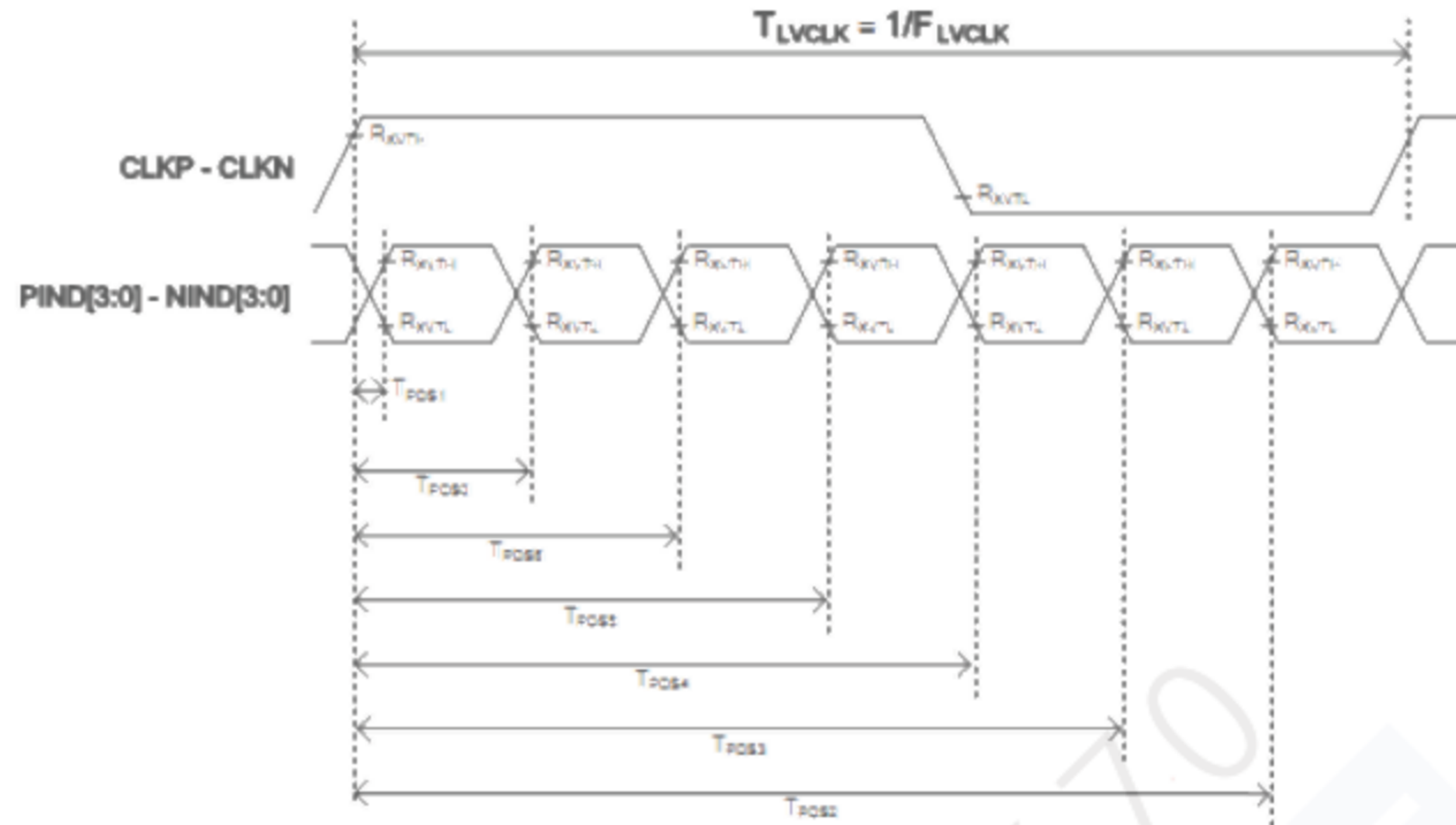
Figure 5.2.3 LVDS input timing
