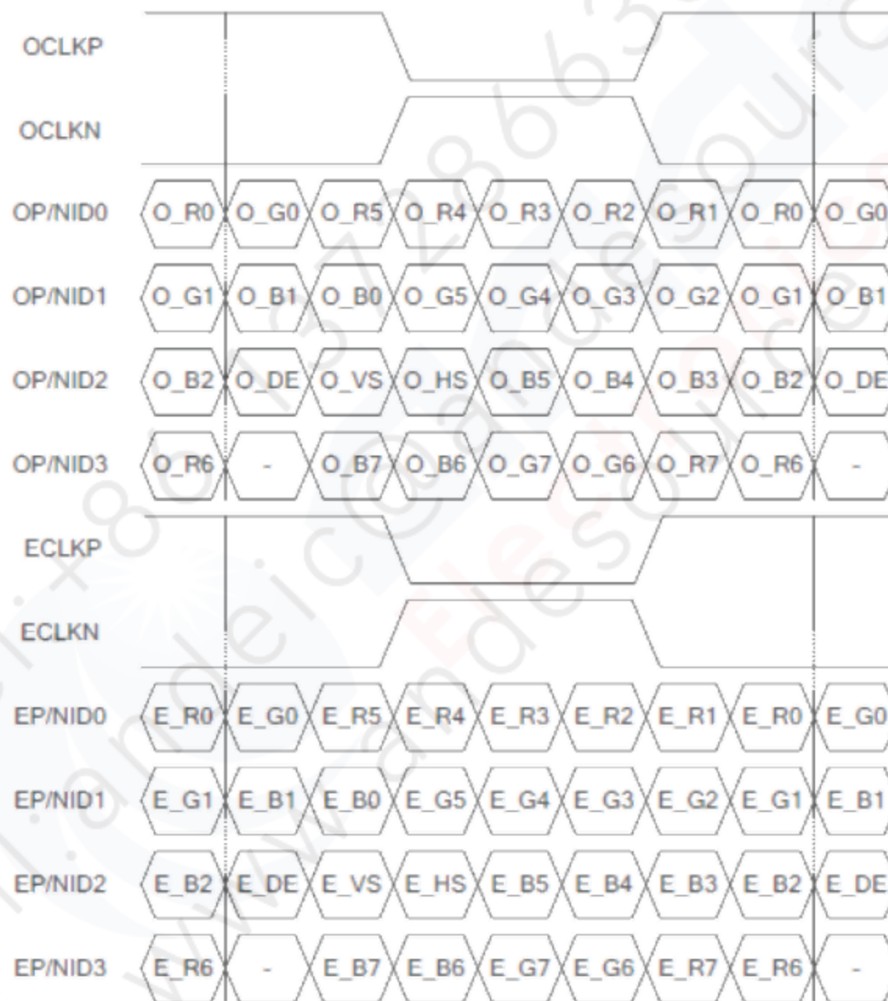
8-bit LVDS Dual Link VESA
