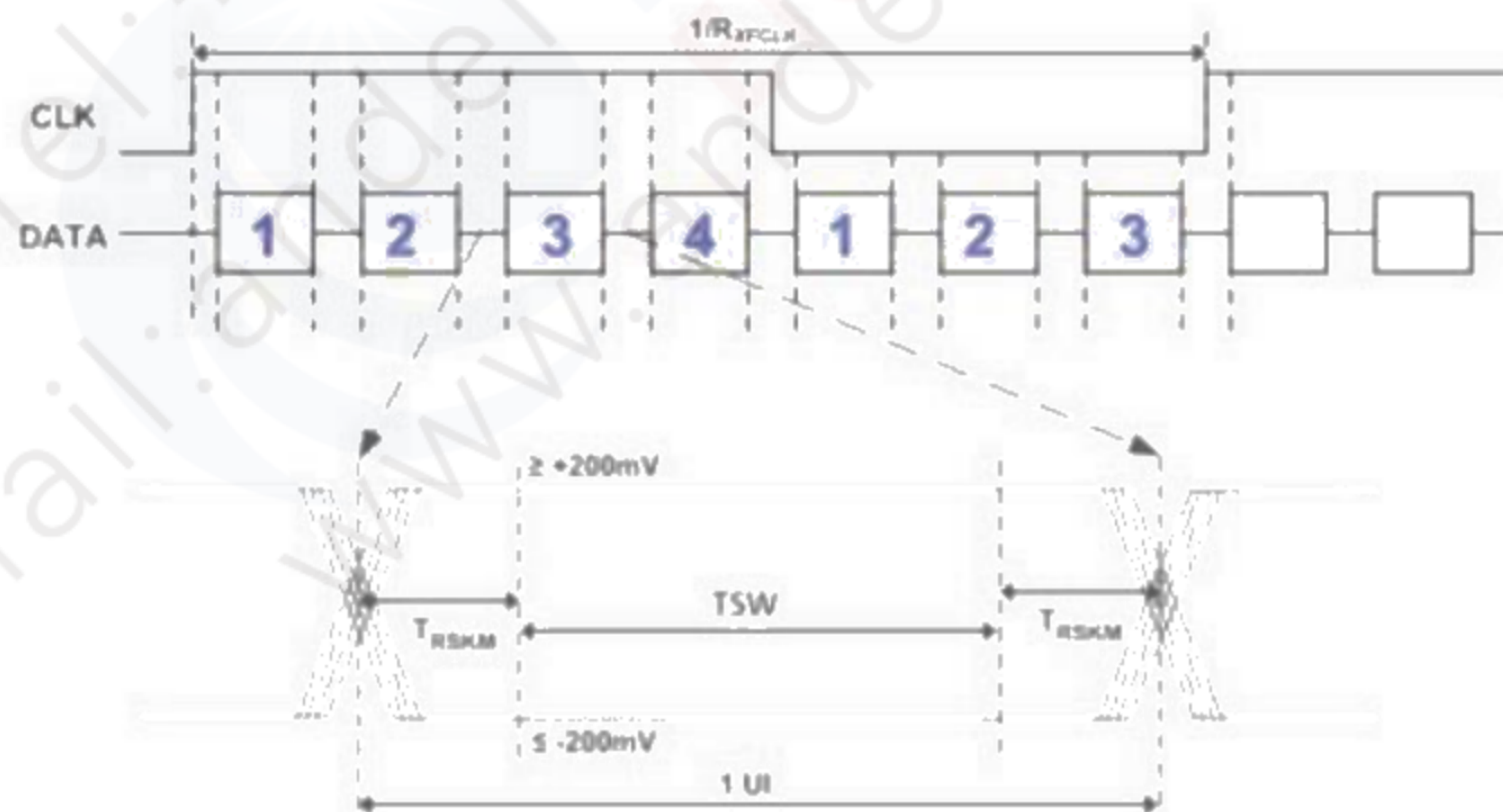
Figure 5.2.2 LVDS Data Skew
