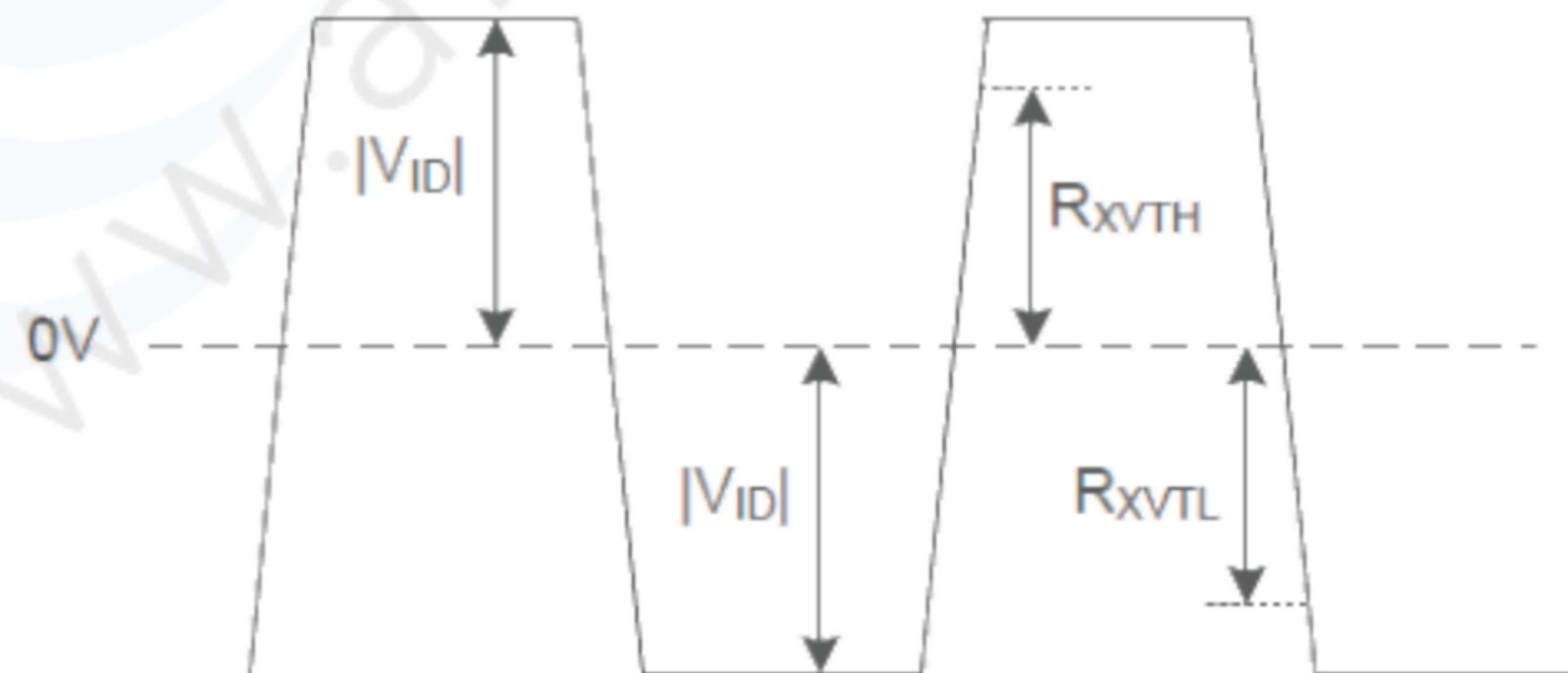
Figure 5.1 LVDS DC Diagram
