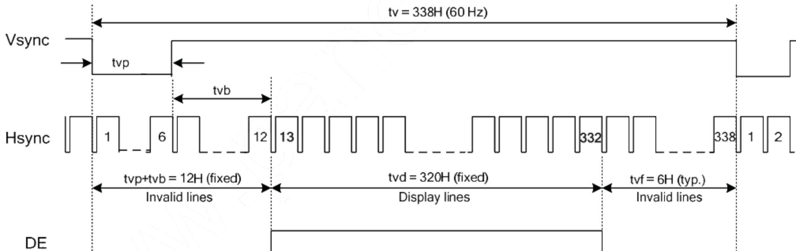
Fig. 9.2 Vertical Timing of Synchronous Mode
