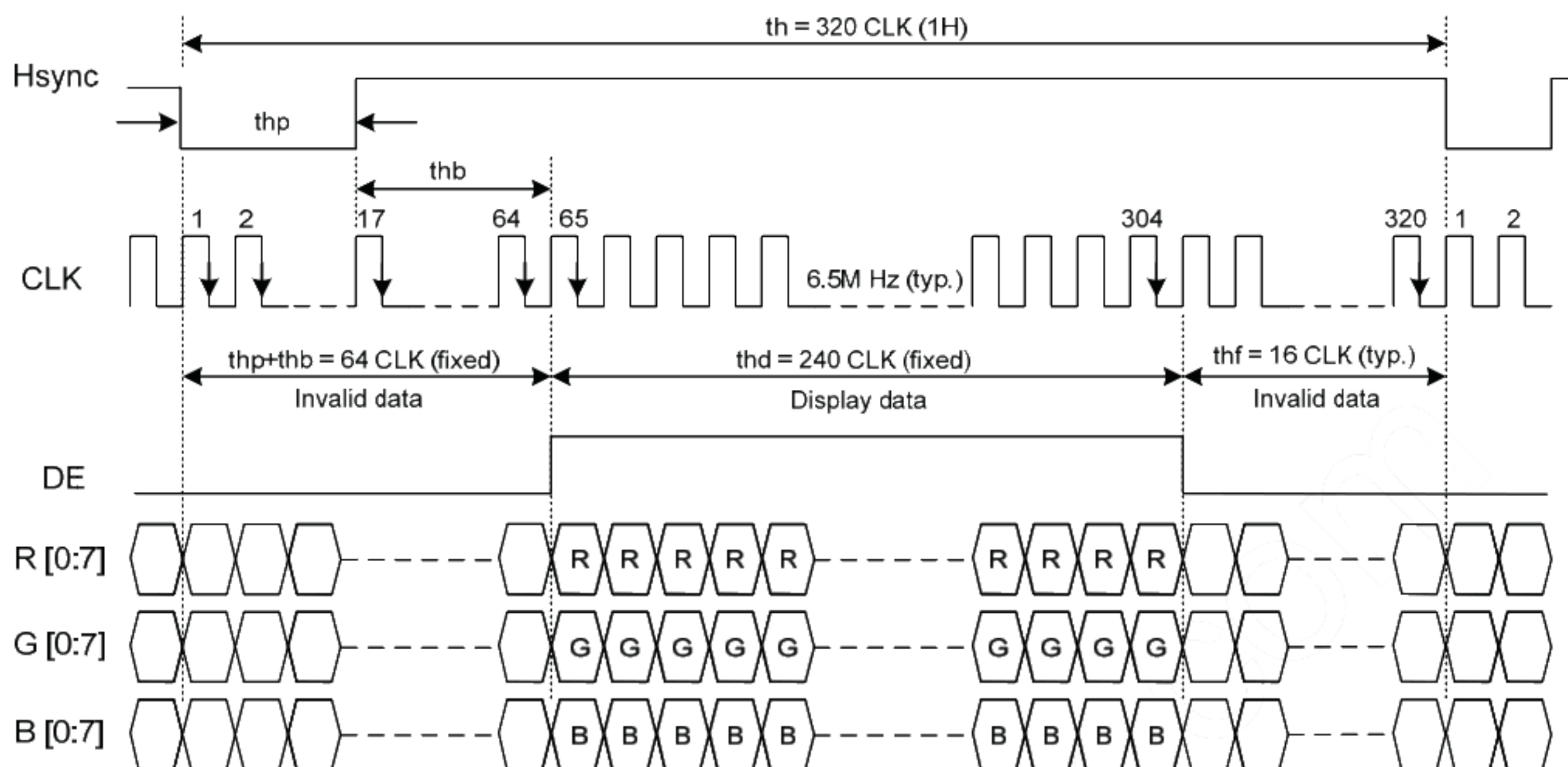
Fig. 9.1 Horizontal Timing of Synchronous Mode
