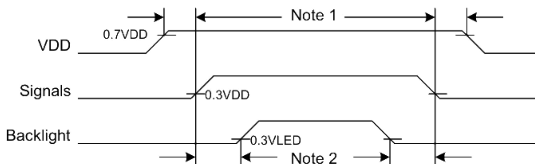
Fig. 9.4 Power Sequence Timing
