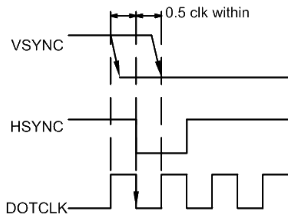
Fig1. VSYNC timing
