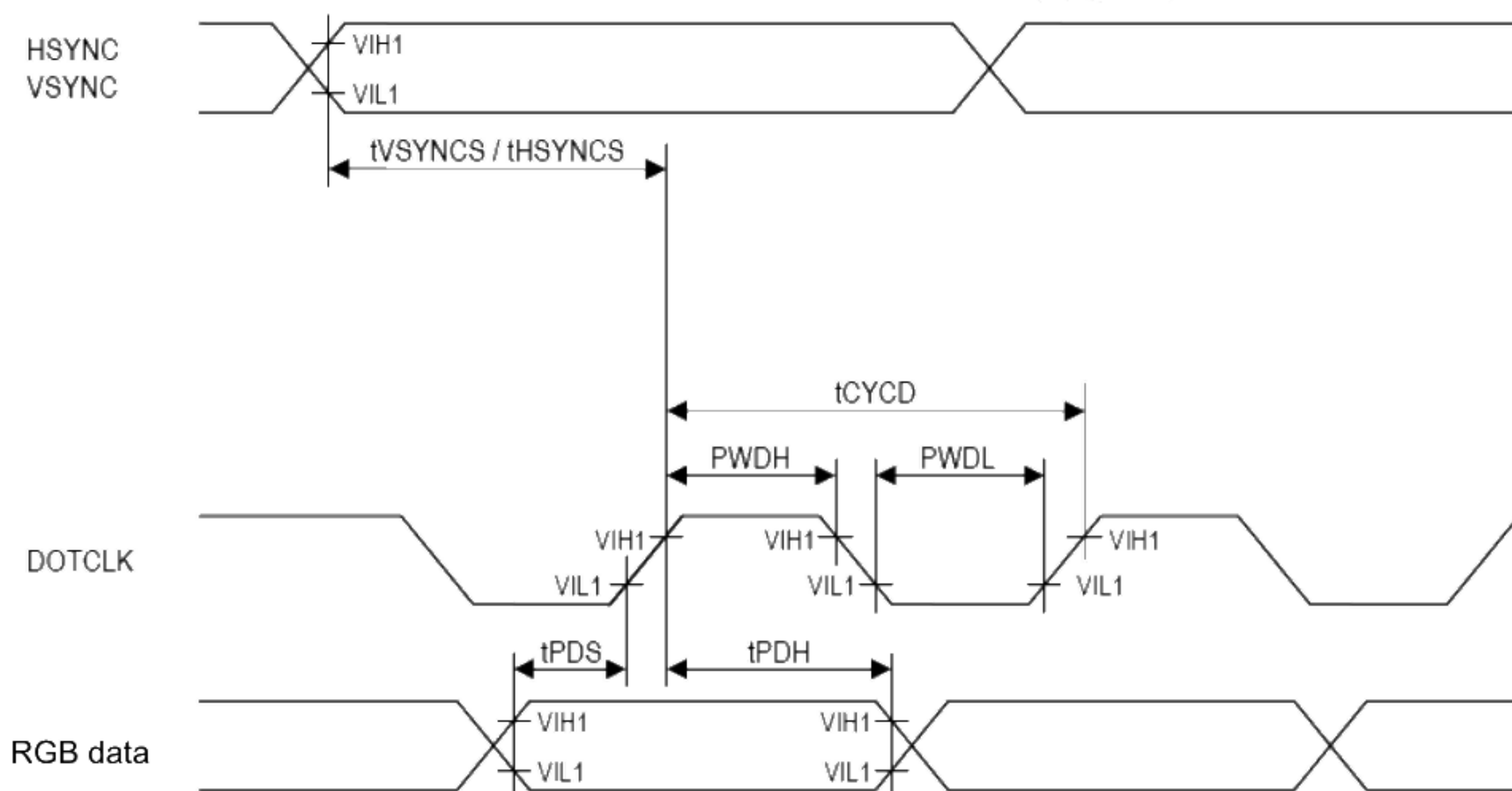
Fig3. RGB Interface timing
