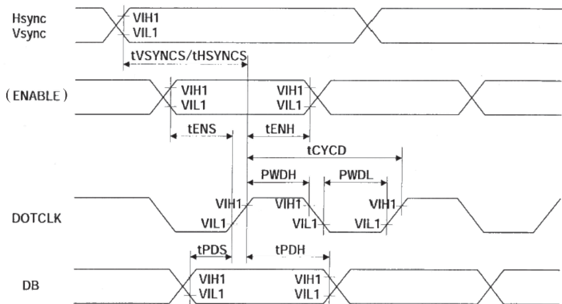
Fig1. RGB Interface timing
