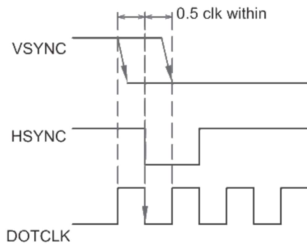
Fig1. VSYNC timing
