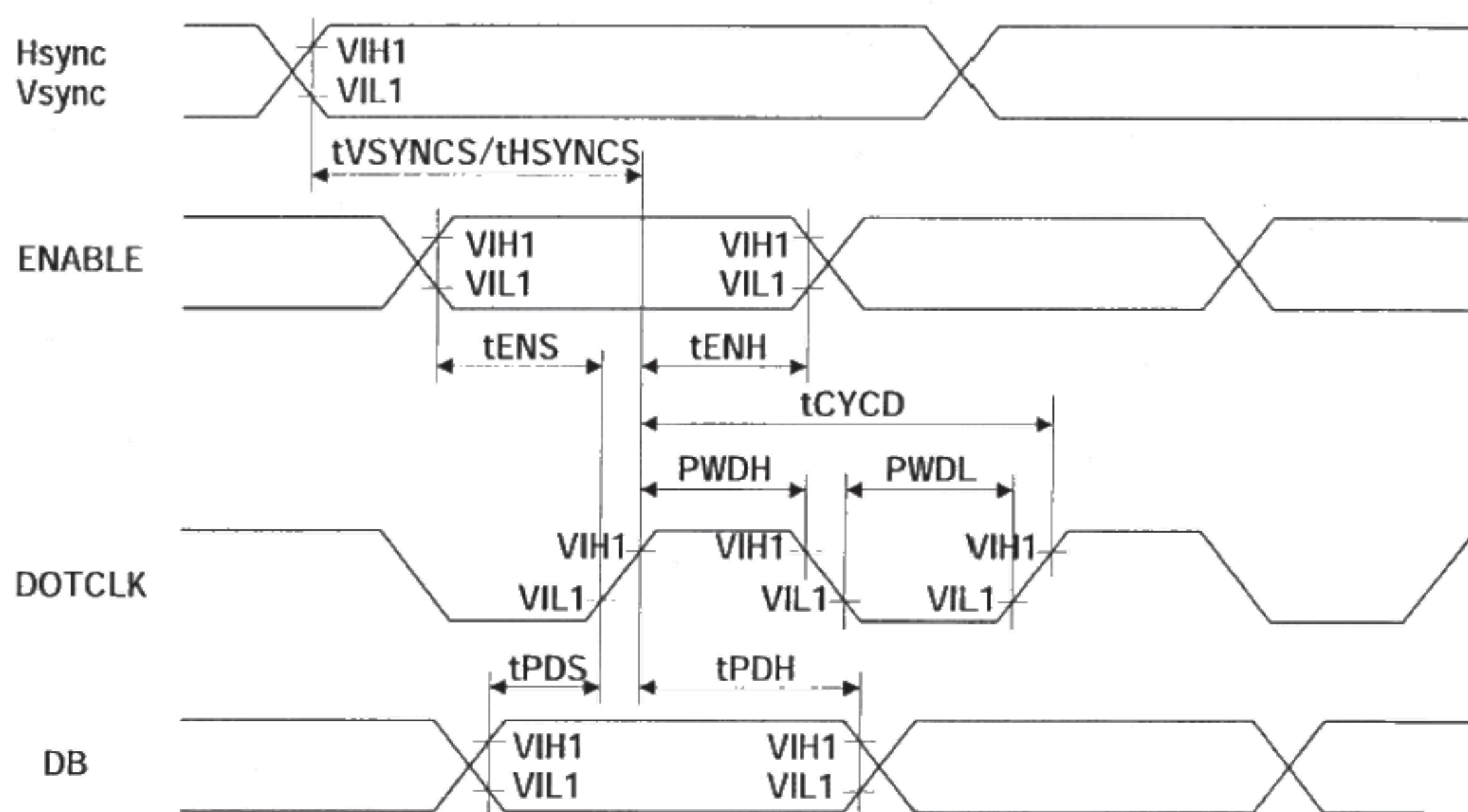
Fig1. RGB Interface timing
