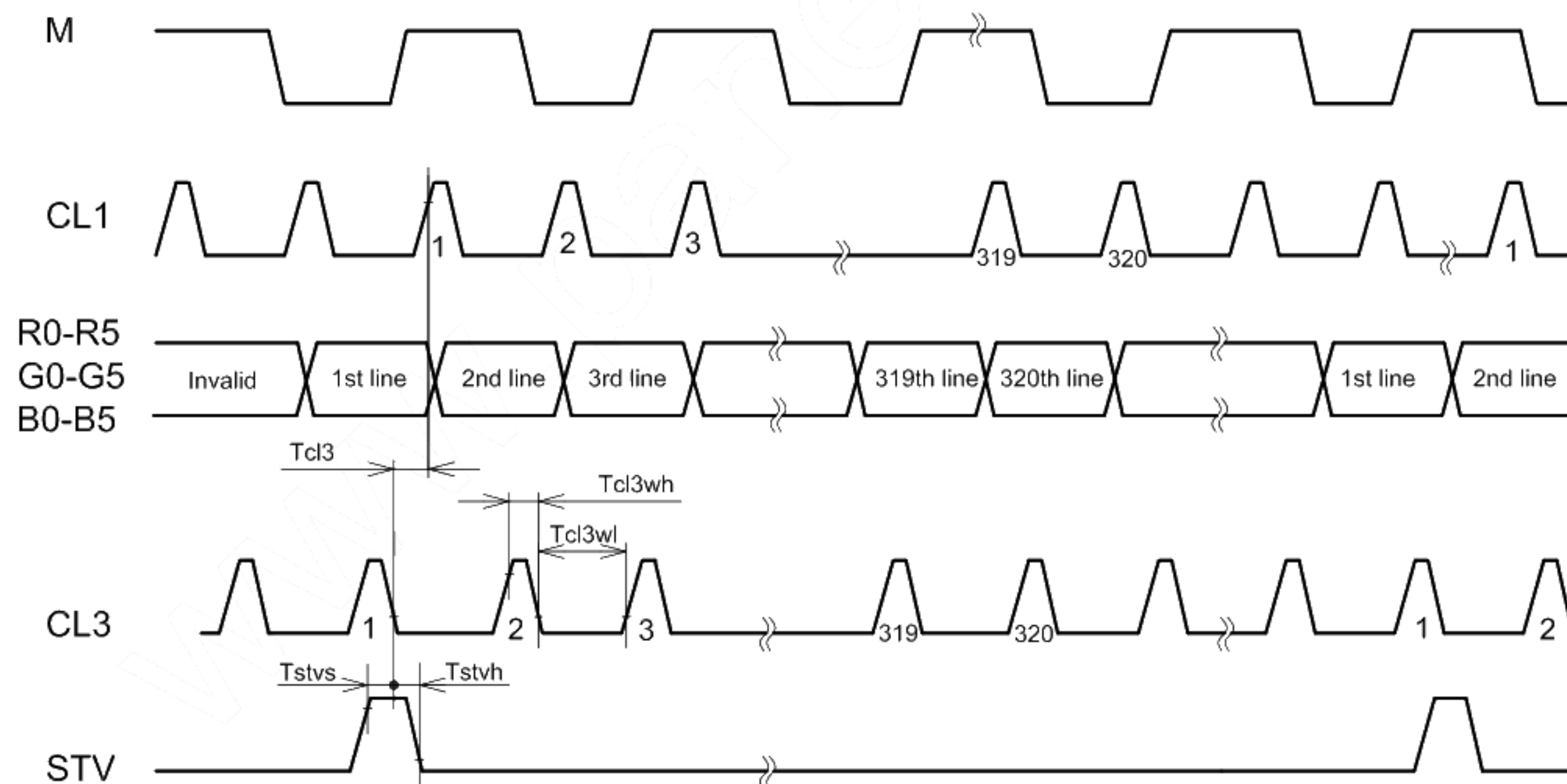
Fig3 . Vertical Timing Sequence for non Tcon
