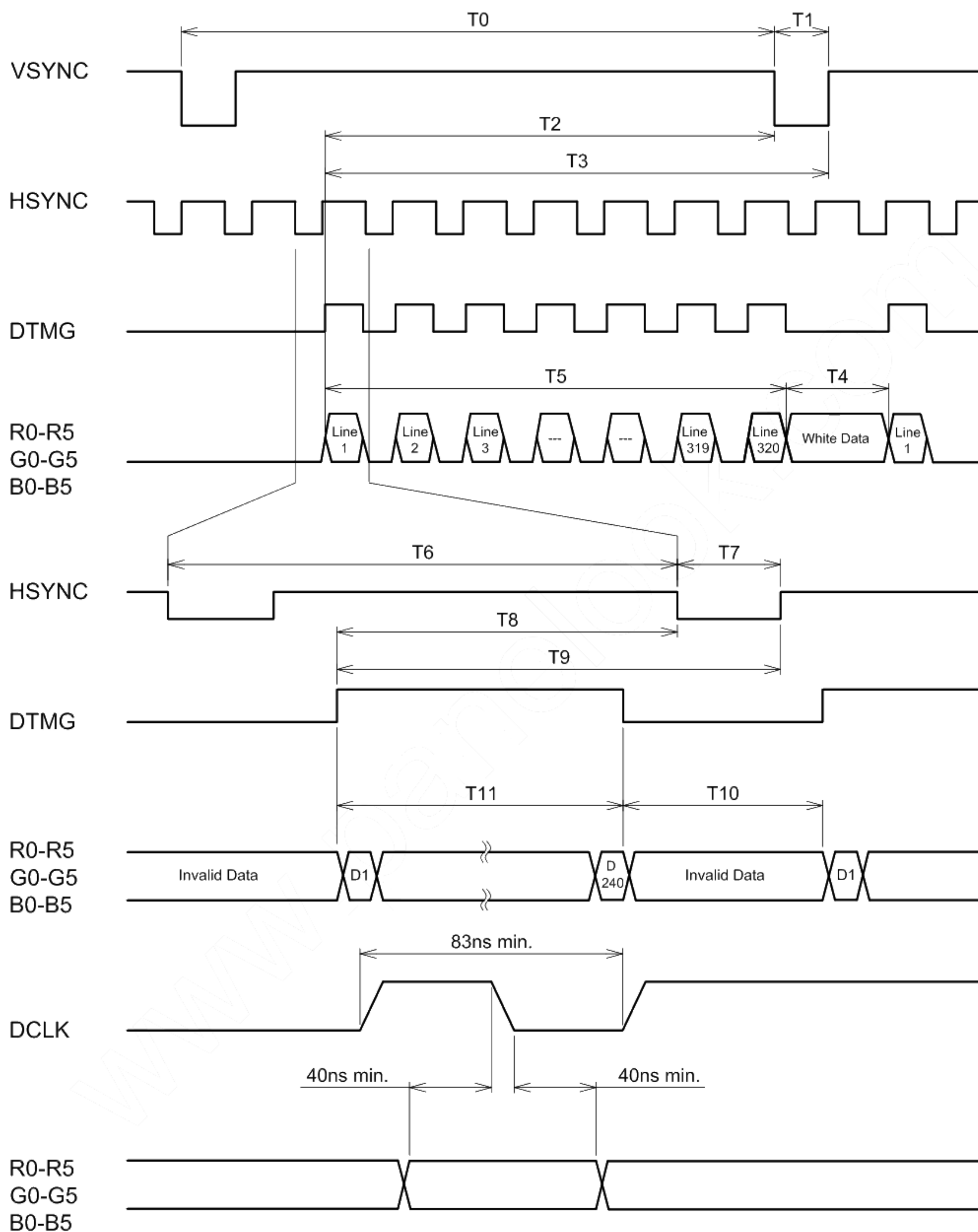
Fig1. Timing sequence for Graphic controller
