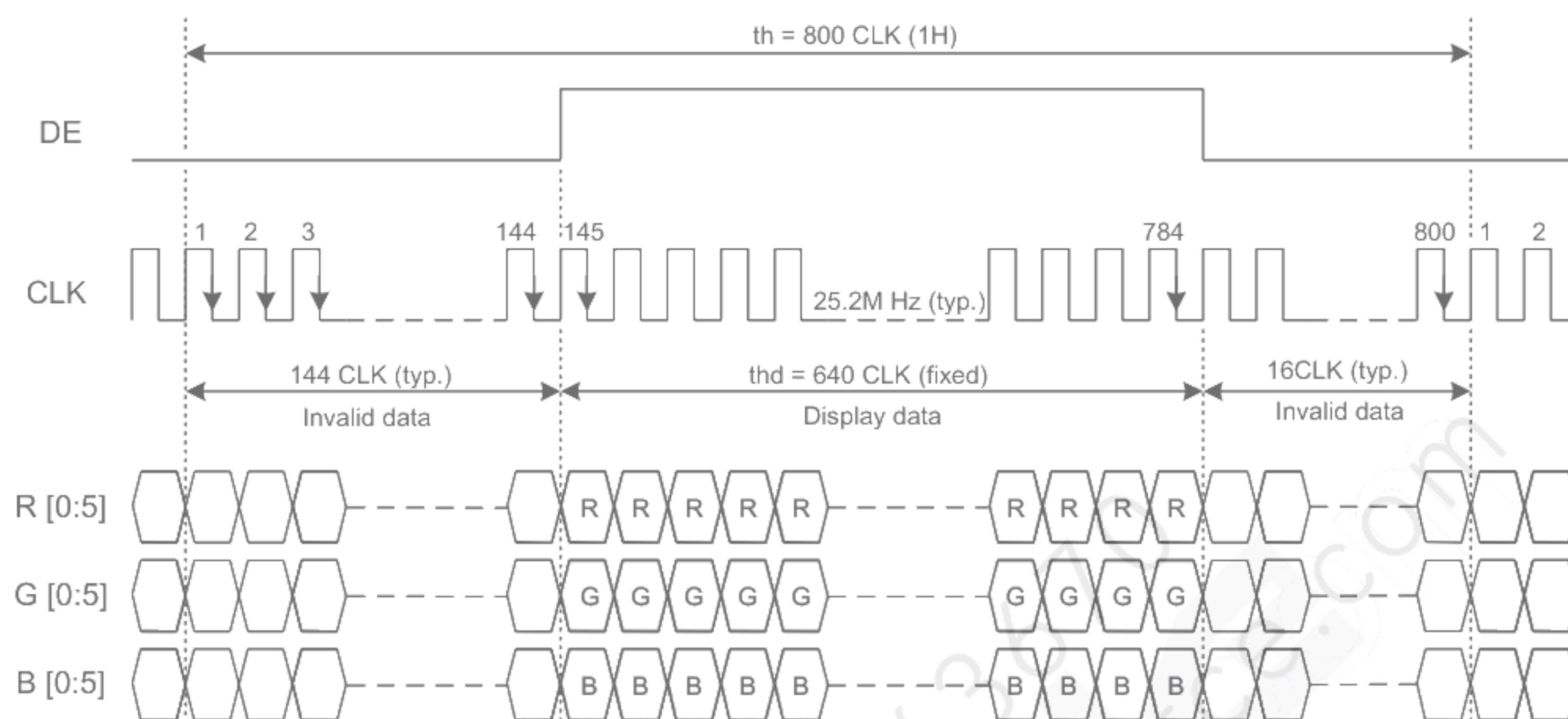
Fig. 9.3 Horizontal Timing of DE Mode
