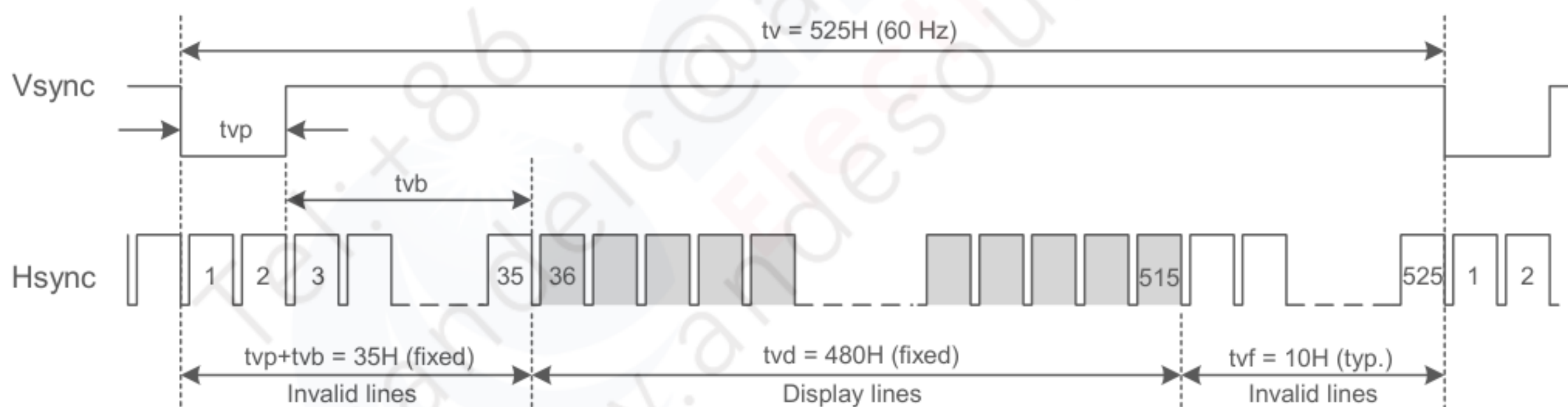
Fig. 9.2 Vertical Timing of Synchronous Mode
