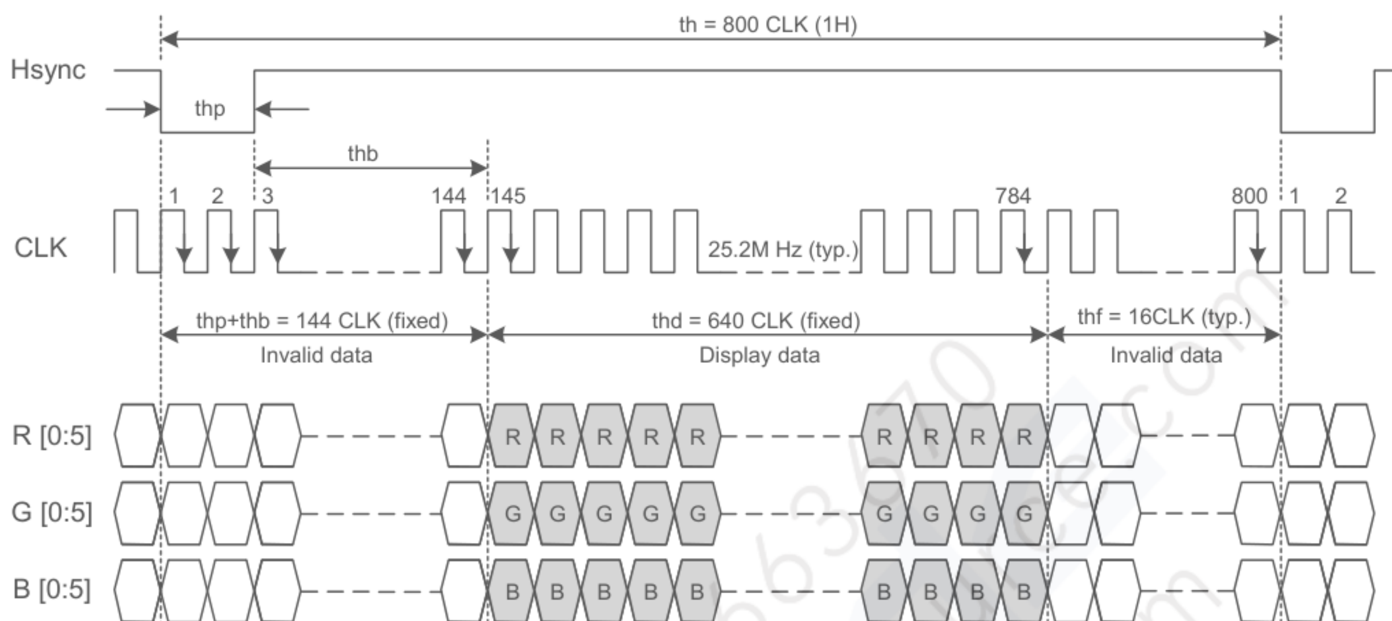
Fig. 9.1 Horizontal Timing of Synchronous Mode
