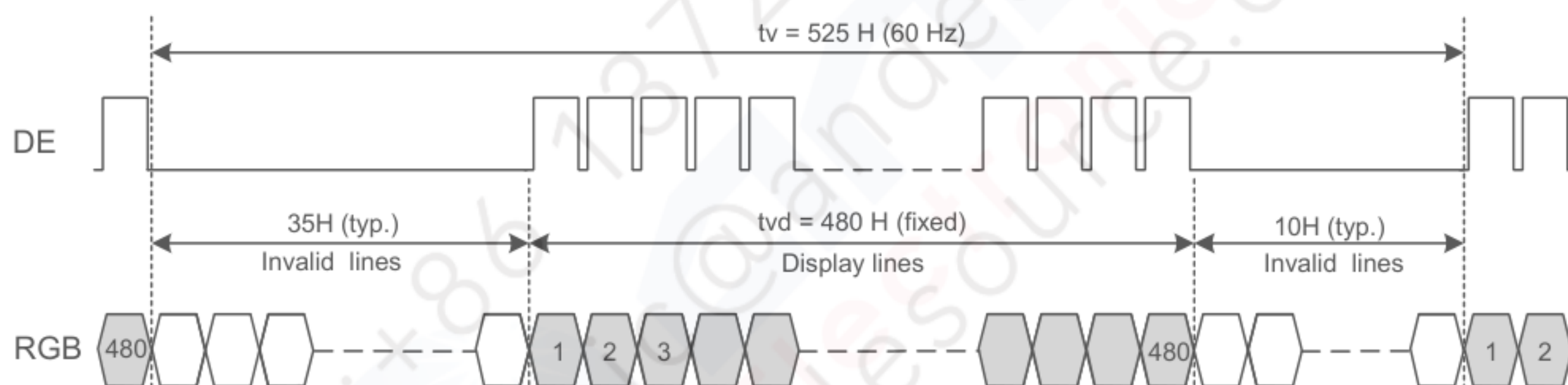
Fig. 9.4 Vertical Timing of DE Mode
