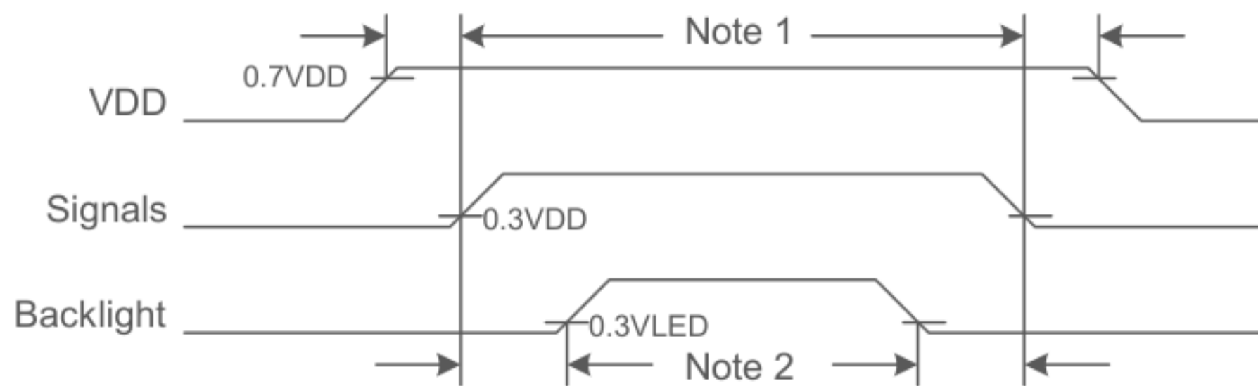
Fig. 9.7 Power Sequence Timing
