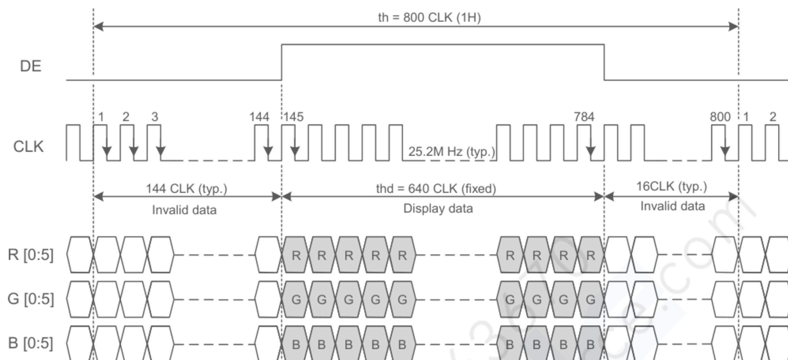
Fig. 9.3 Horizontal Timing of DE Mode
