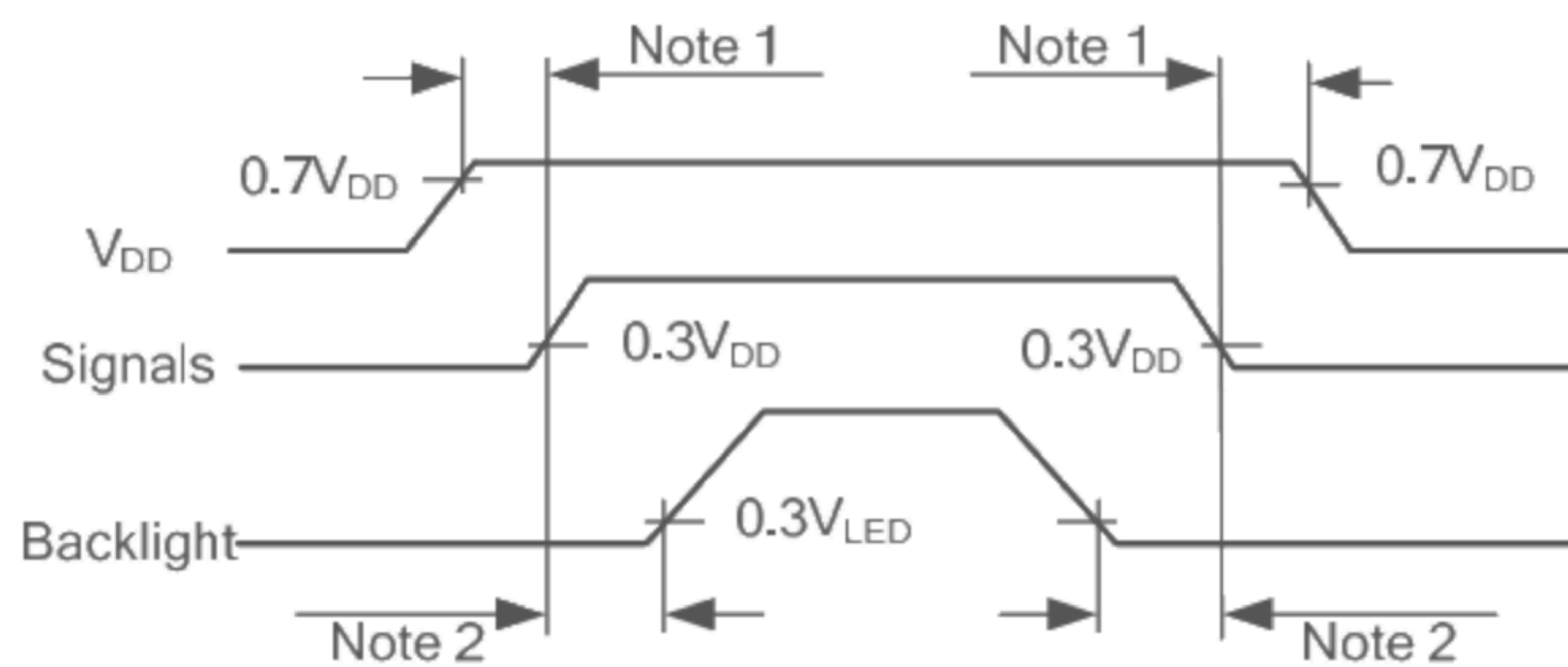
Fig. 9.4 Power Sequence Timing
