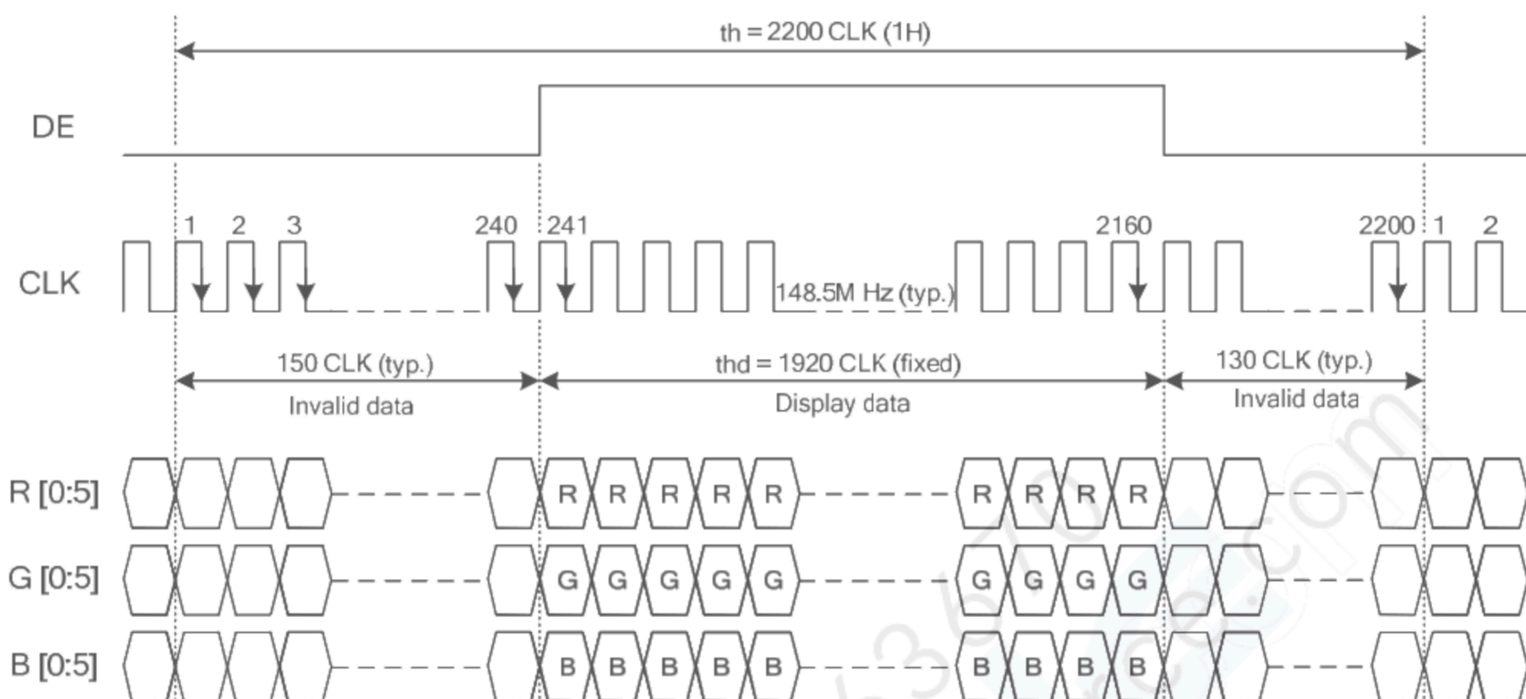
Fig. 9.1 Horizontal Timing
