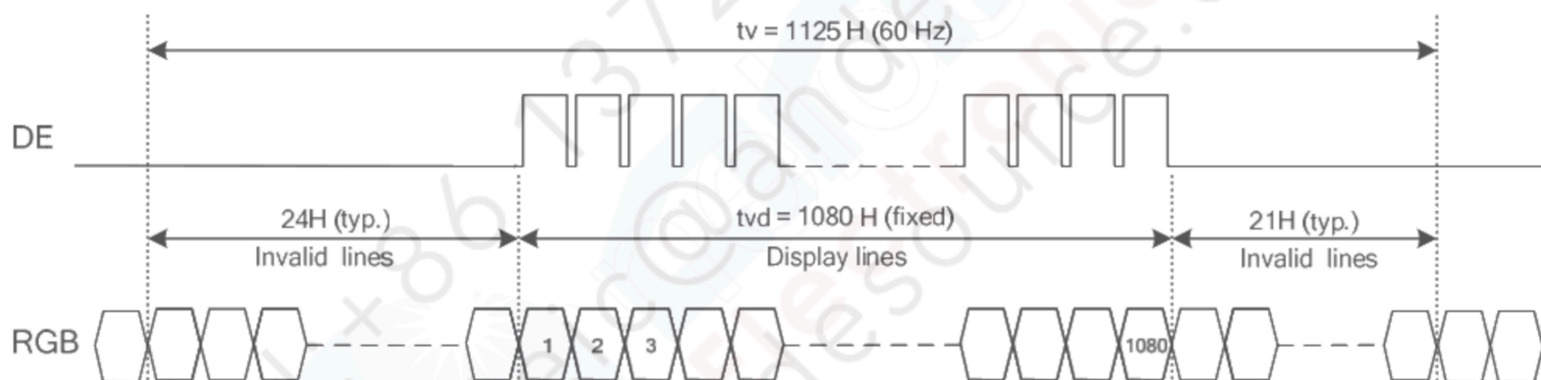
Fig. 9.2 Vertical Timing
