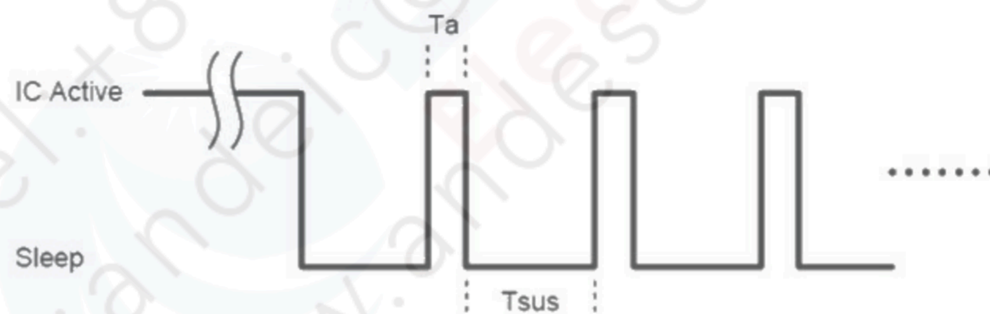
Fig. 11.2 Idle Sequence Diagram
