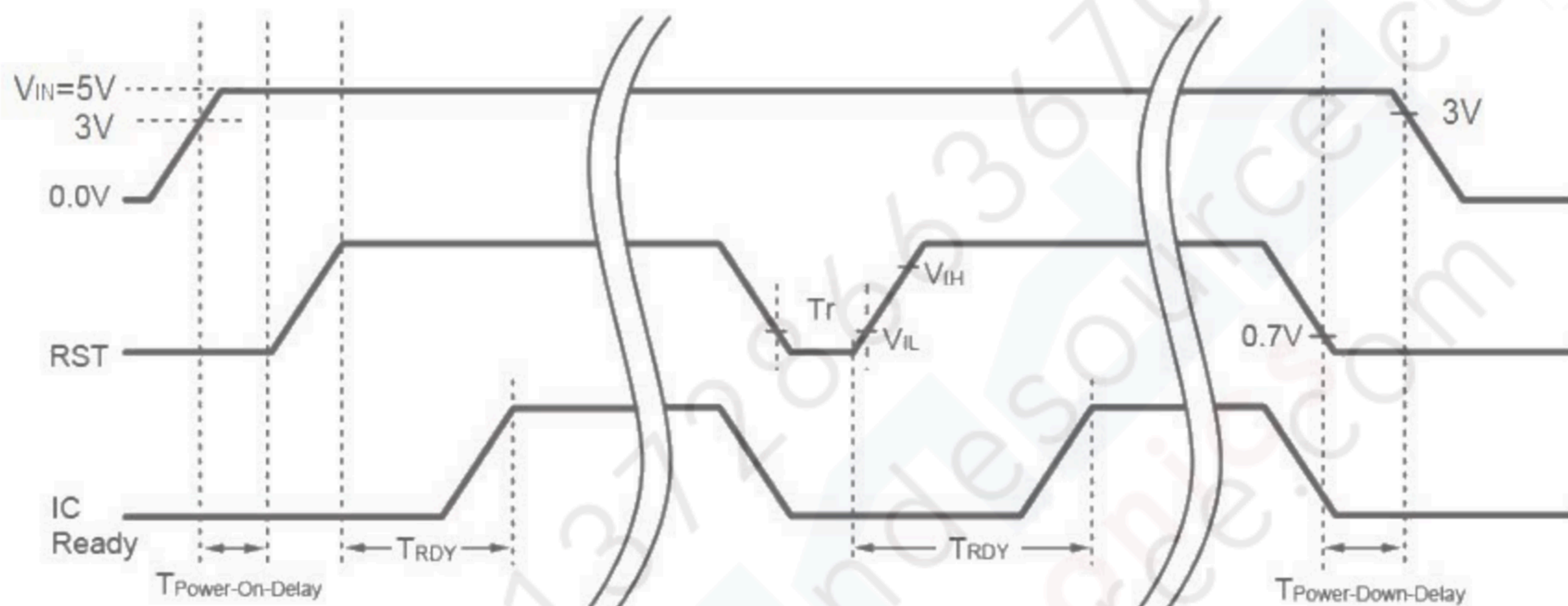
Fig. 11.1 Power On Sequence Diagram
