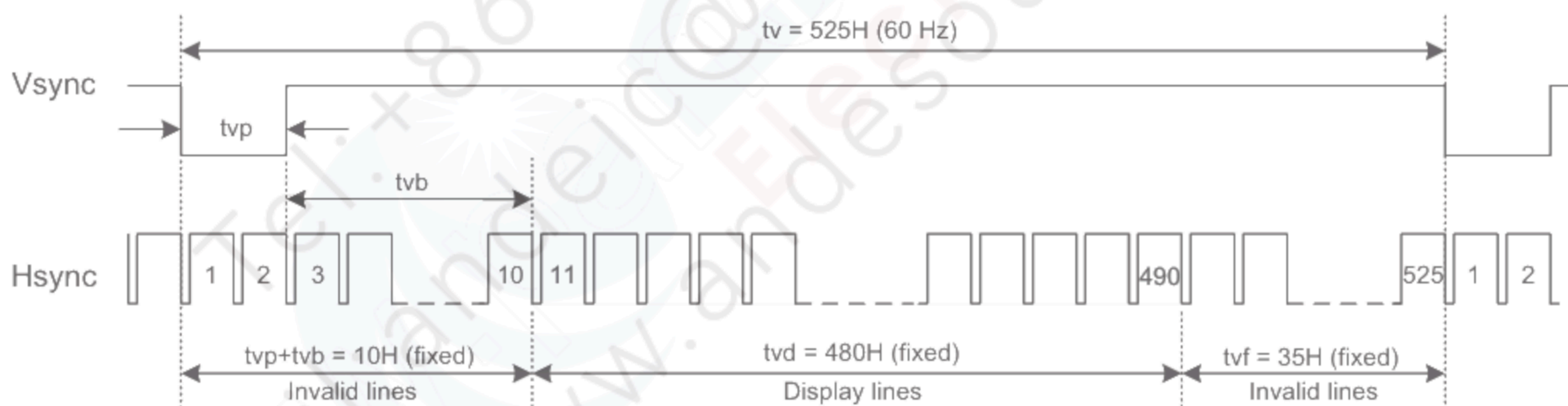
Fig. 9.2 Vertical Timing
