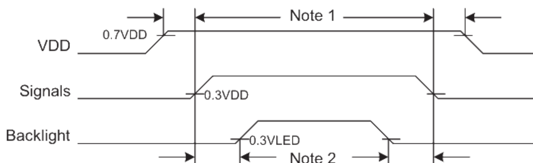
Fig. 8.7 Power Sequence Timing
