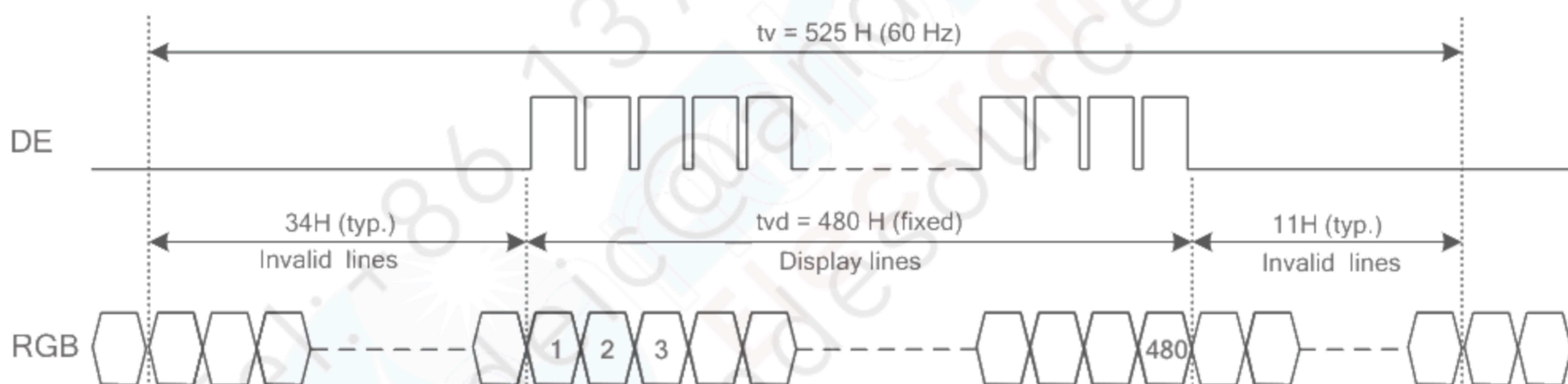
Fig. 9.2 Vertical Timing
