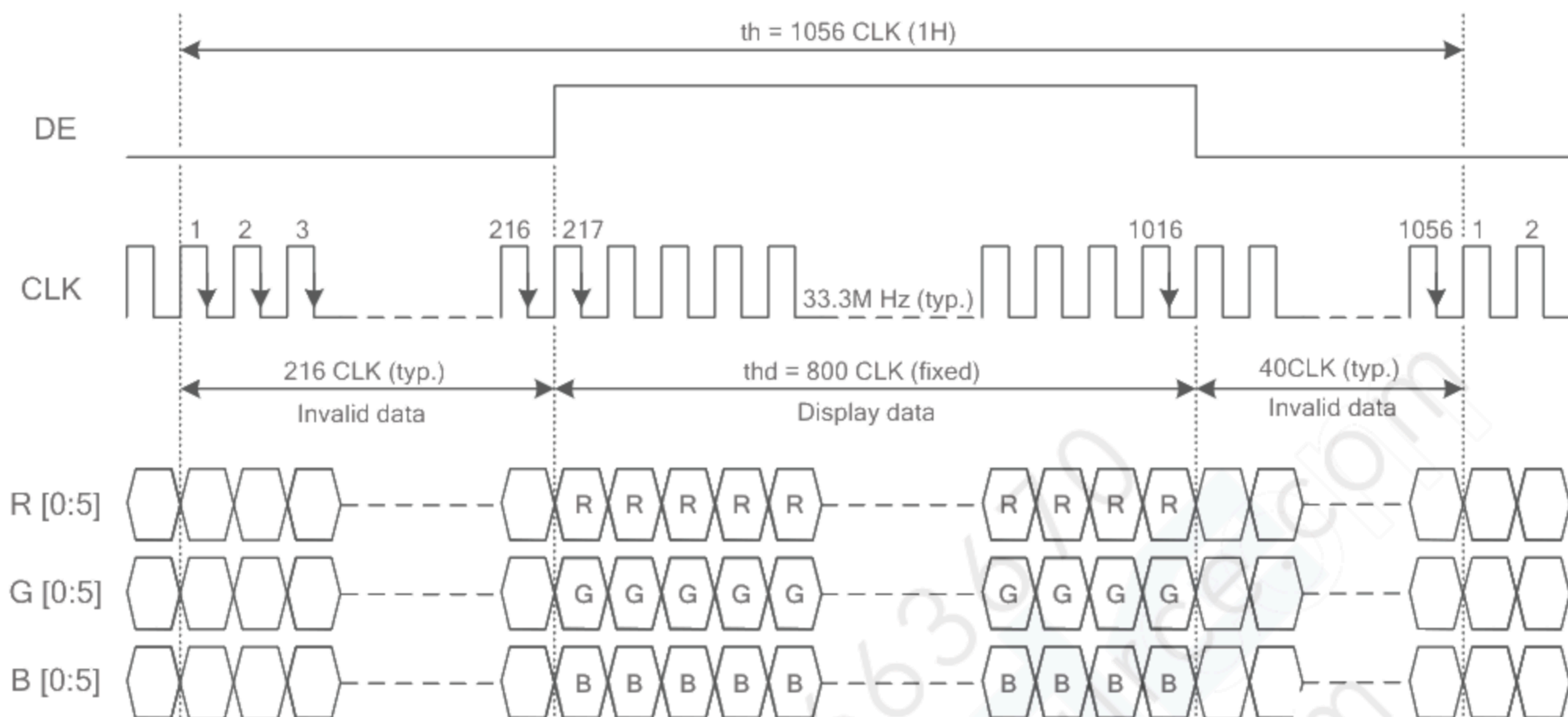
Fig. 9.1 Horizontal Timing
