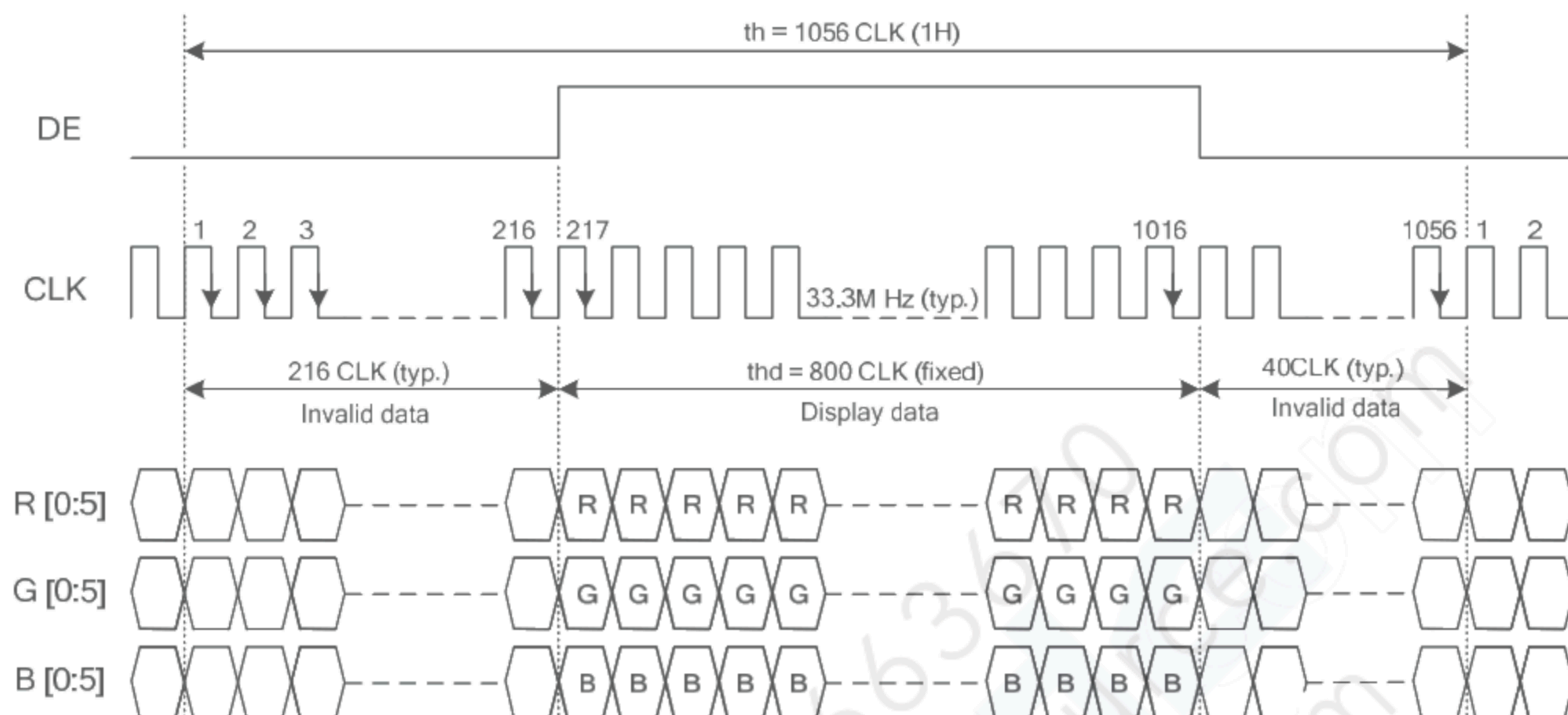
Fig. 9.1 Horizontal Timing
