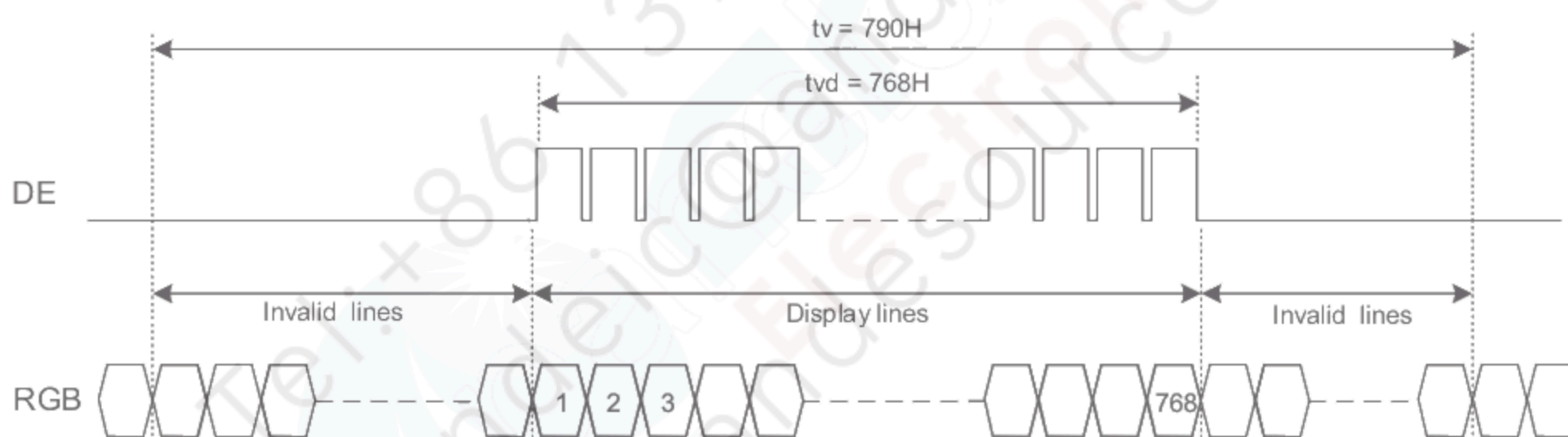
Fig. 9.2 Vertical Timing
