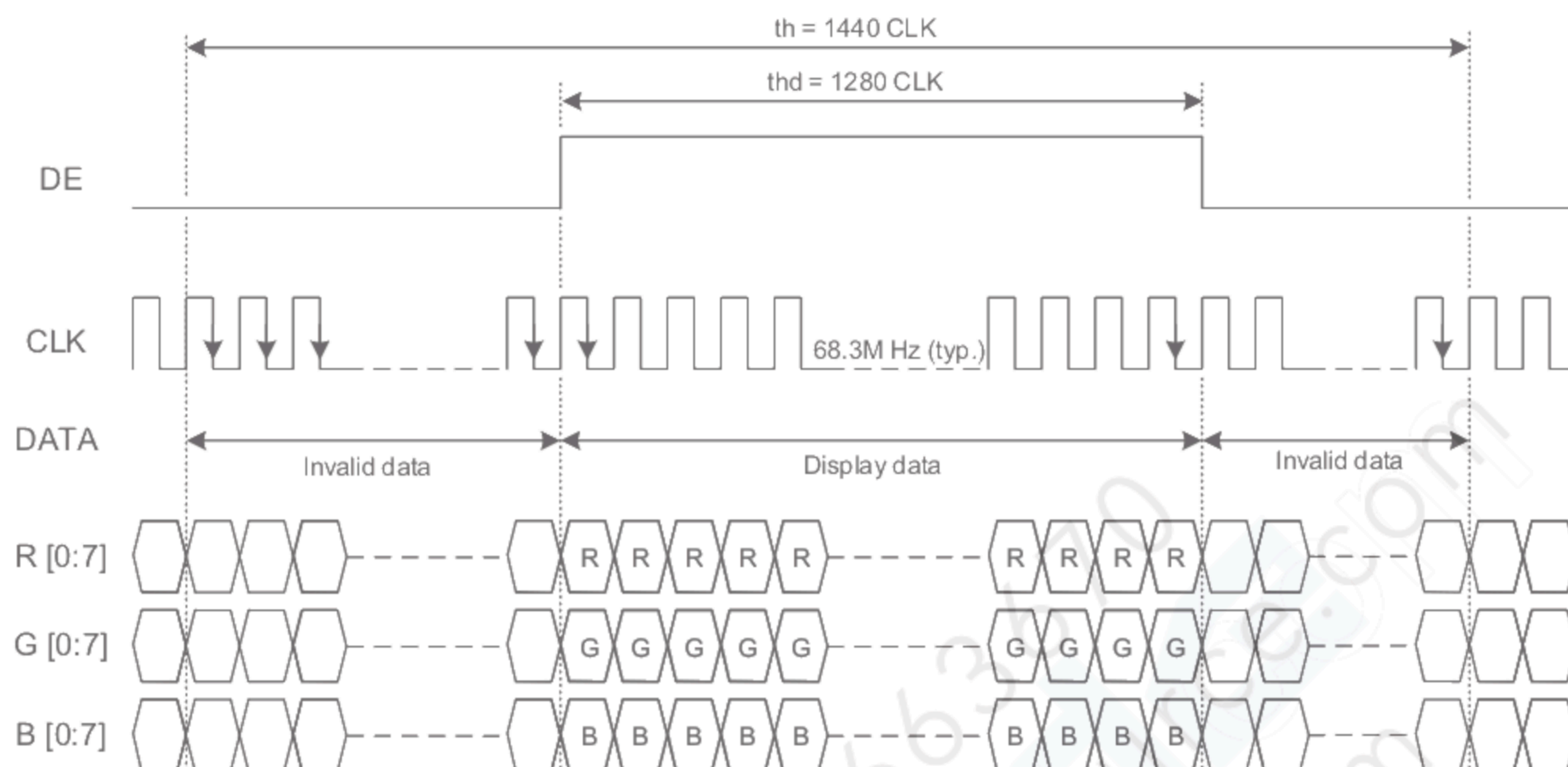
Fig. 9.1 Horizontal Timing
