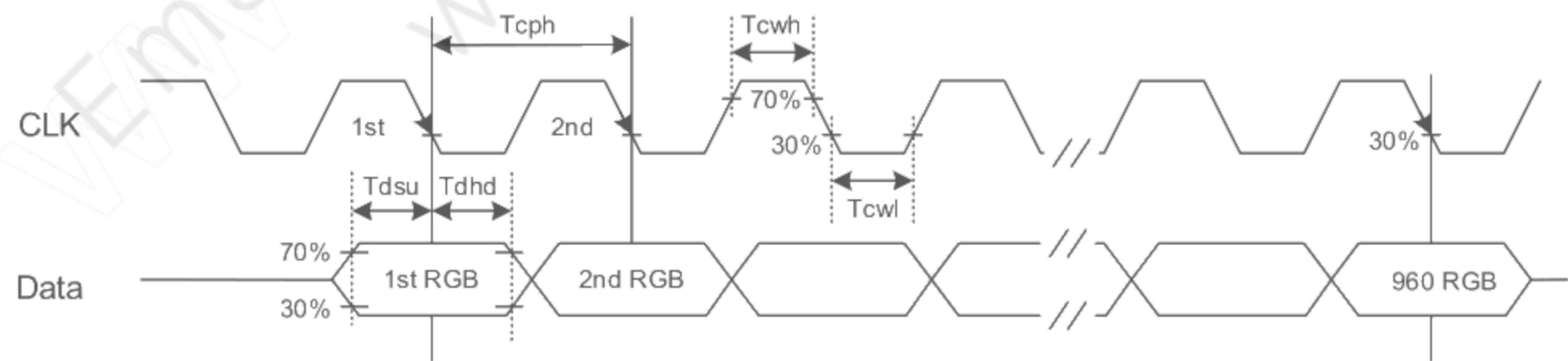
Fig. 9.3 Setup & Hold Time
