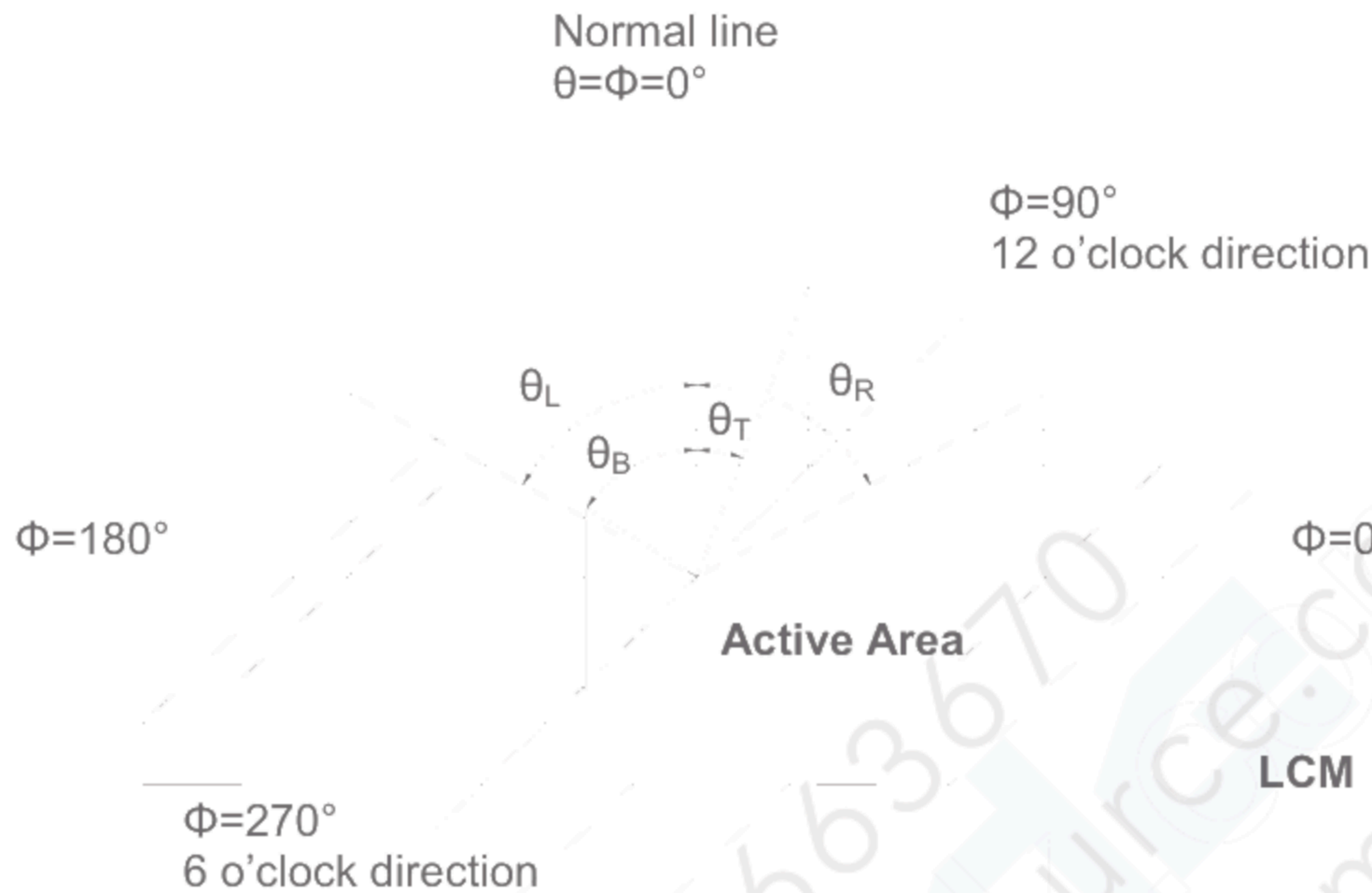
Fig. 4-1 Definition of viewing angle
