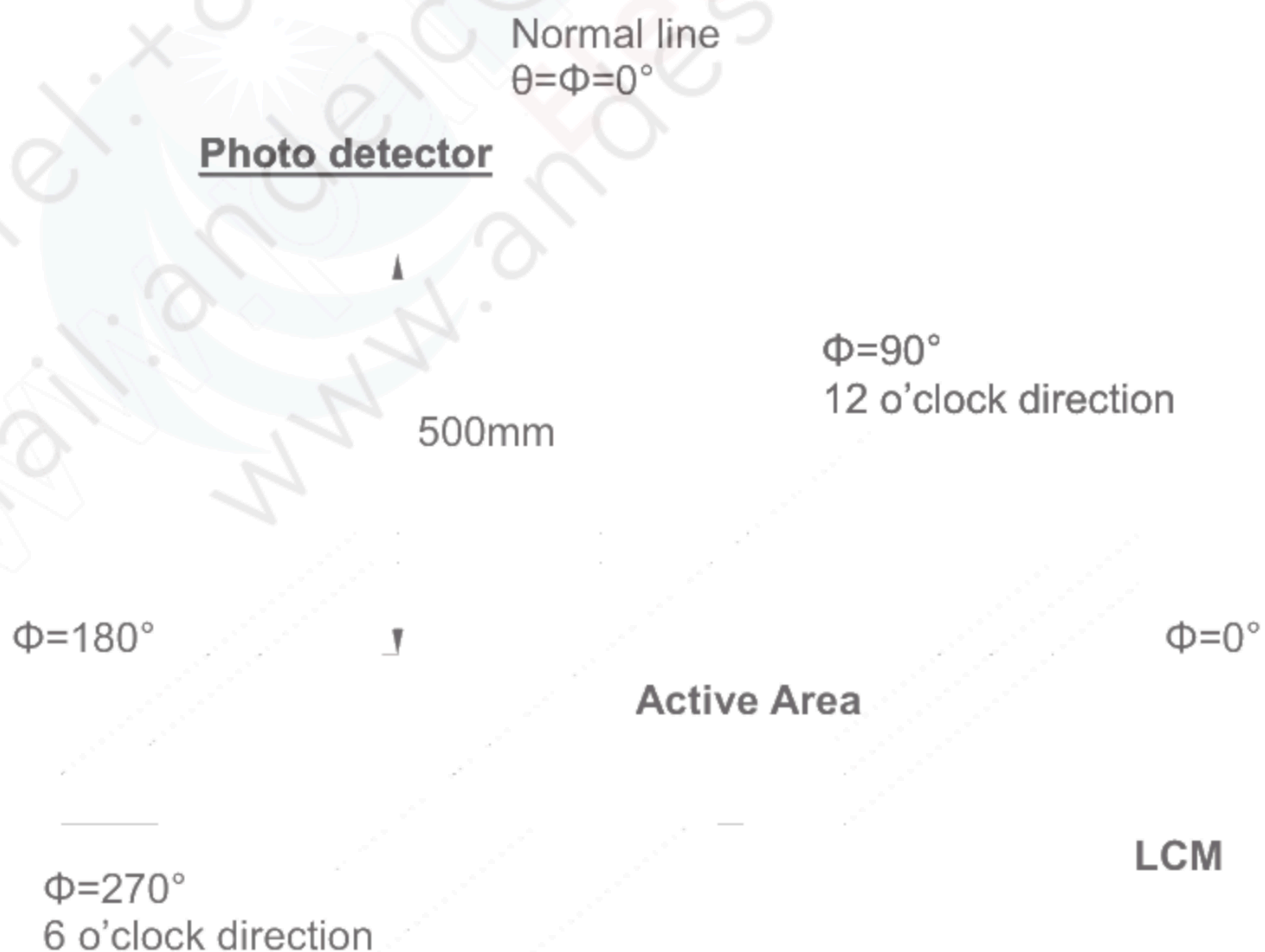
Fig. 4-2 Optical measurement system setup
