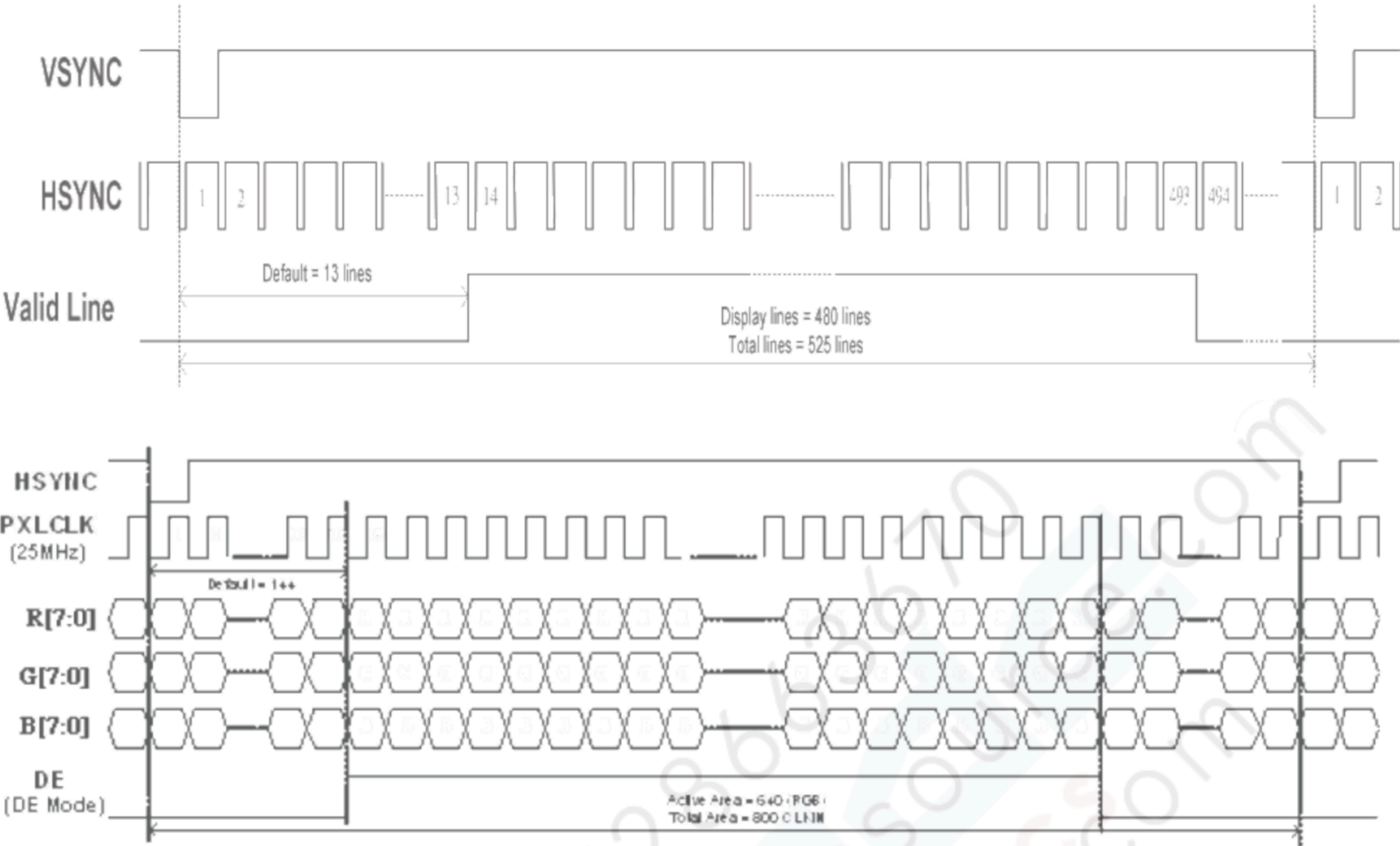
Fig. 3-4 24 bit RGB mode for 640 x (RGB) x 480
