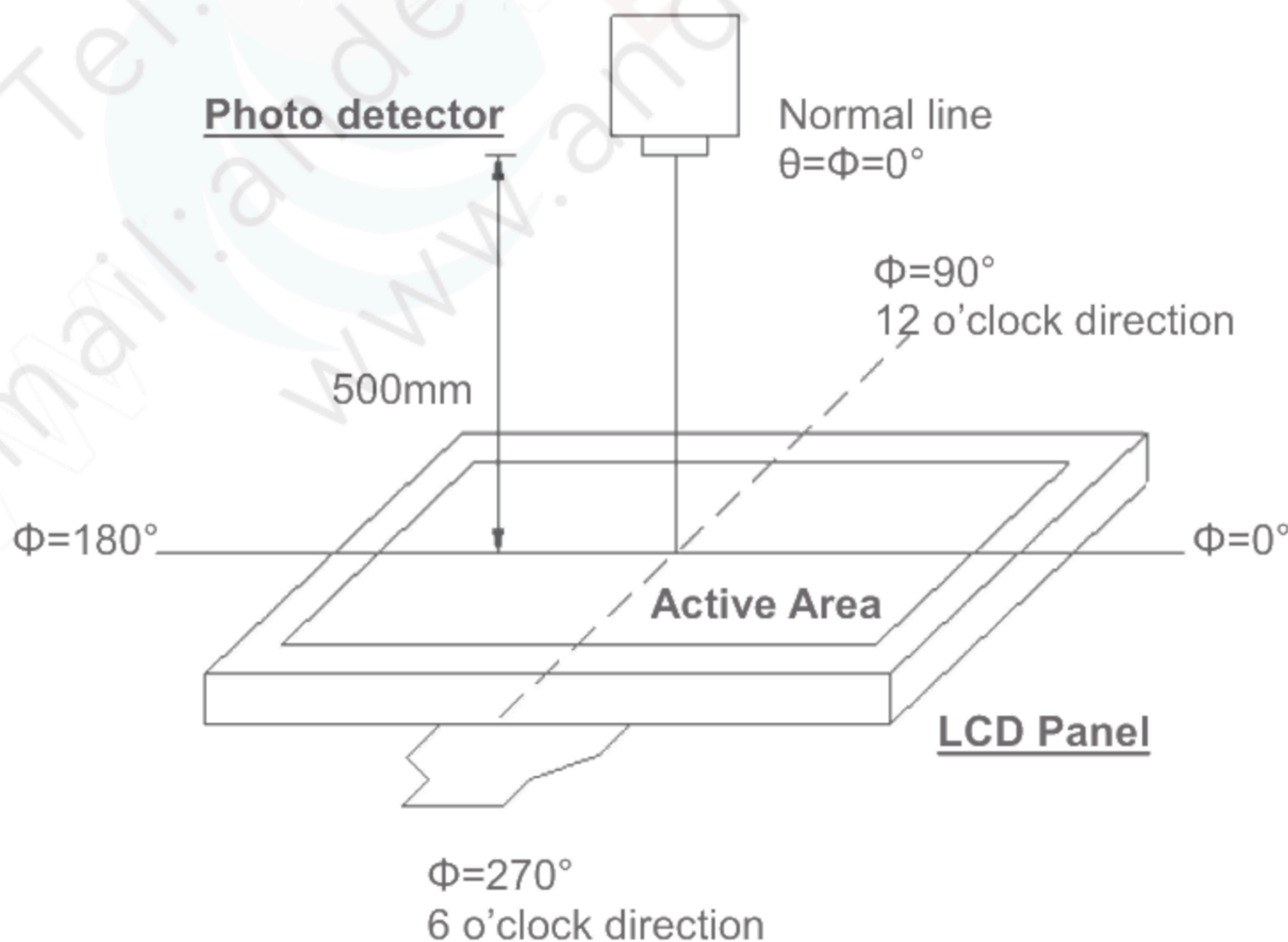
Fig. 4-2 Optical measurement system setup
